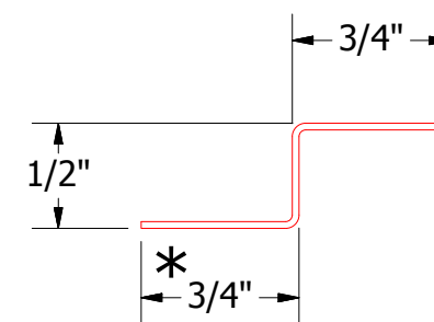
MFA681-Support Z
