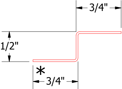
MFA681-Support Z
