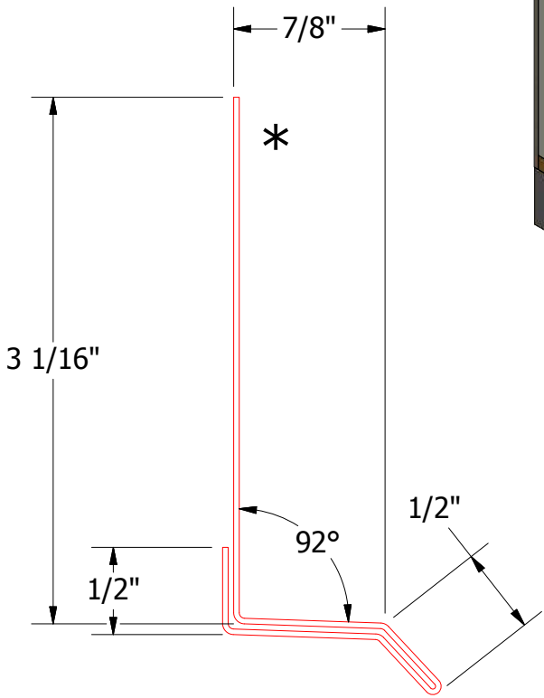
MFA-Base Trim
