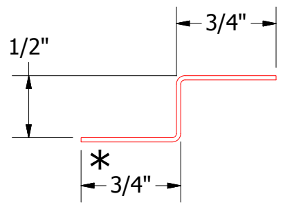
MFA681-Support Z
