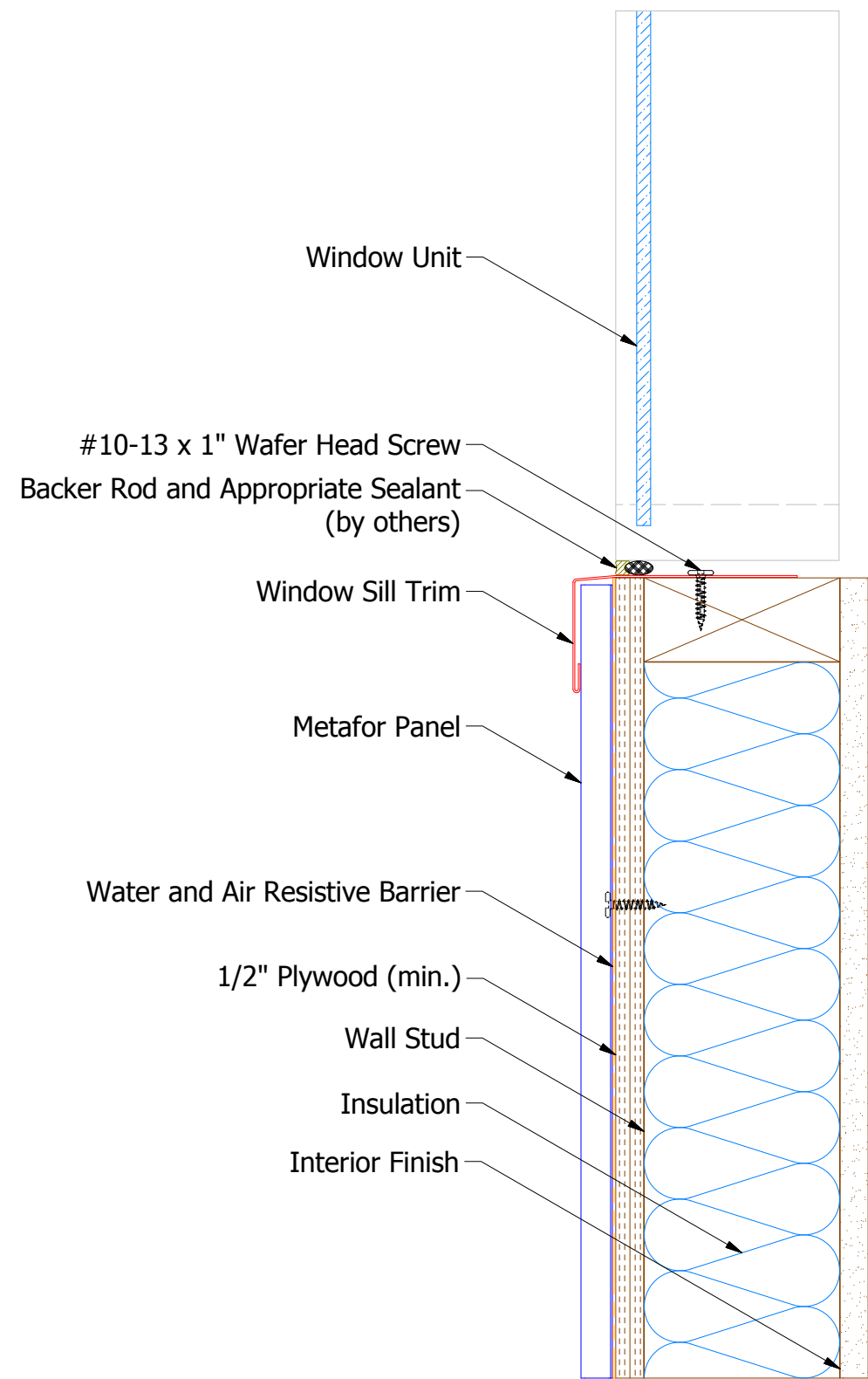
Vertical Application
