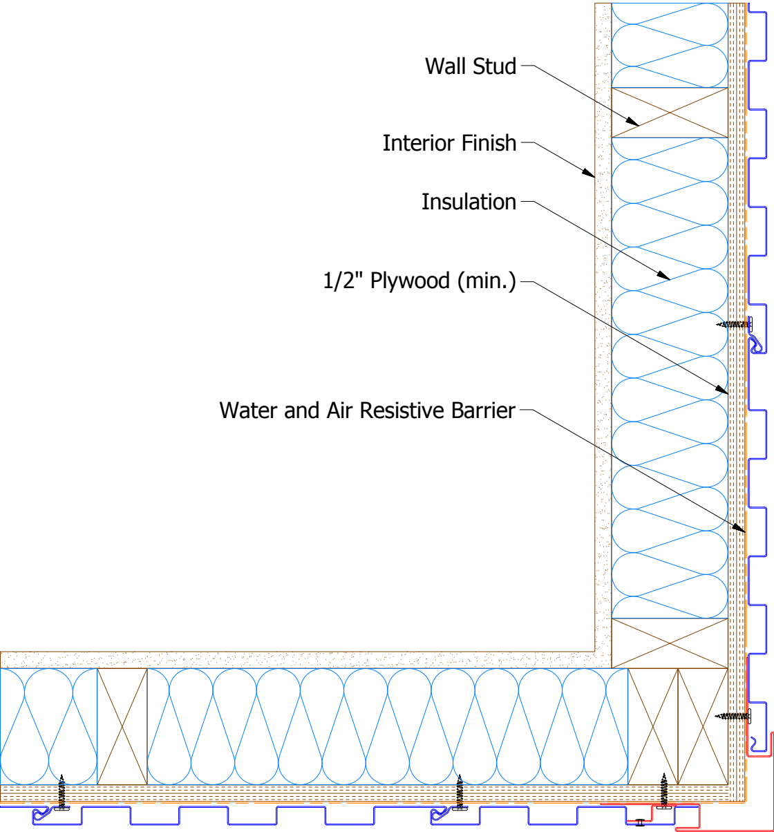
Vertical Application
