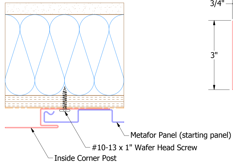
Starting Application
