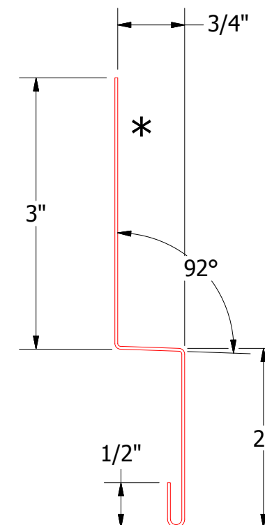
MFA671-Head Trim
