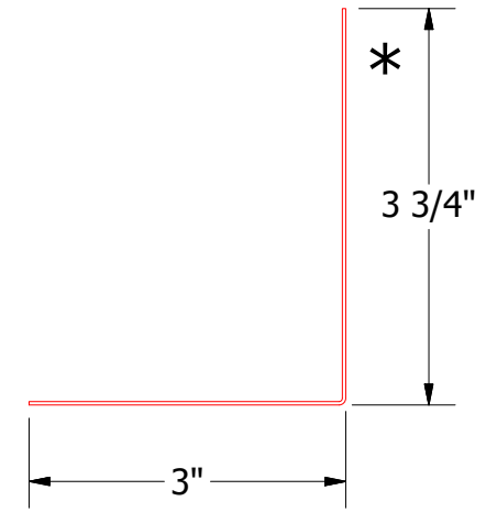
MFAXXX-Angle Trim
