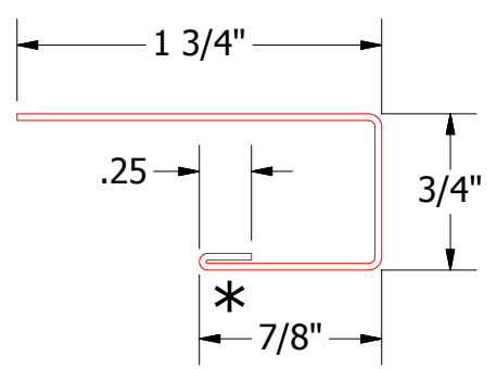
MFA034-J Channel
