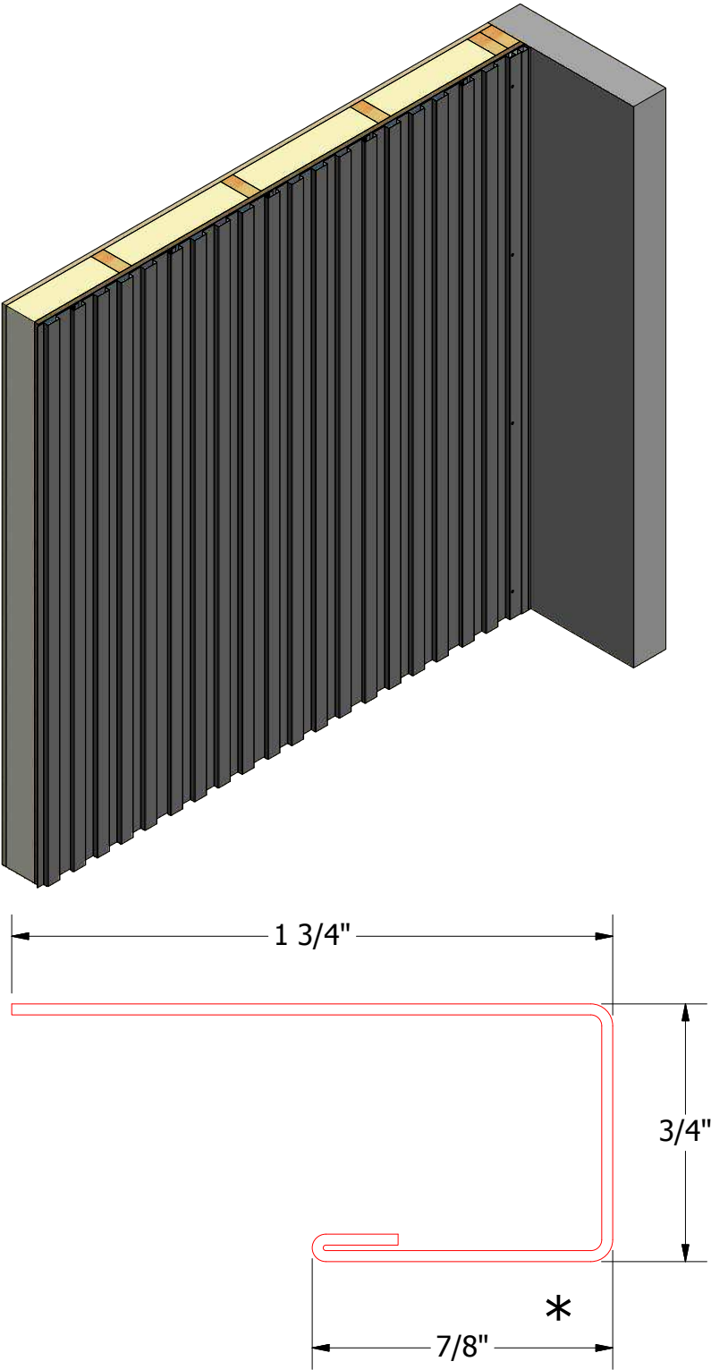
MFA034-J Channel
