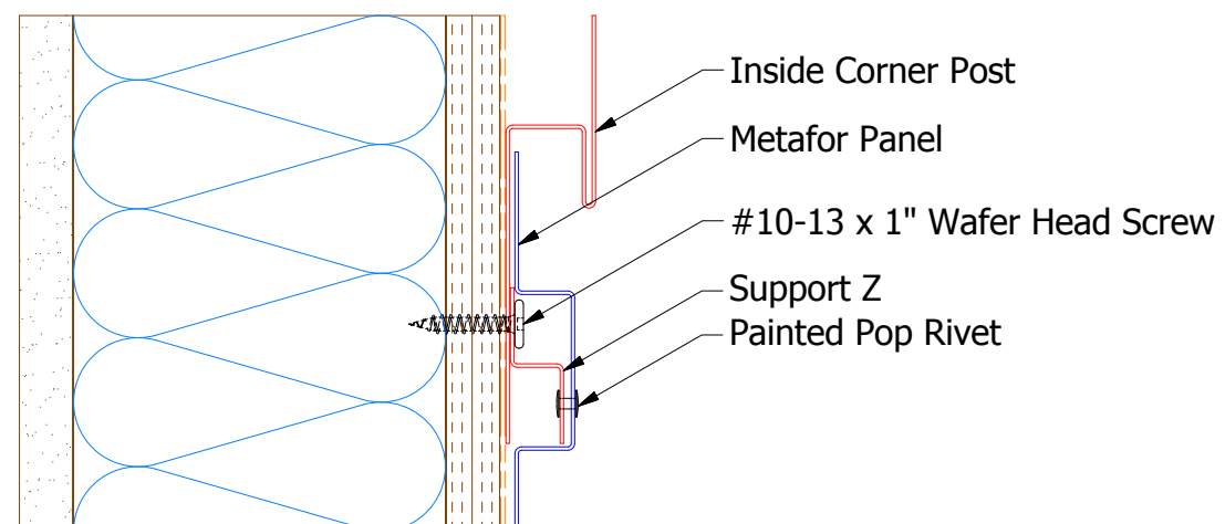
Ending Application
