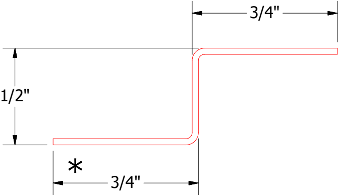
MFA681-Support Z
