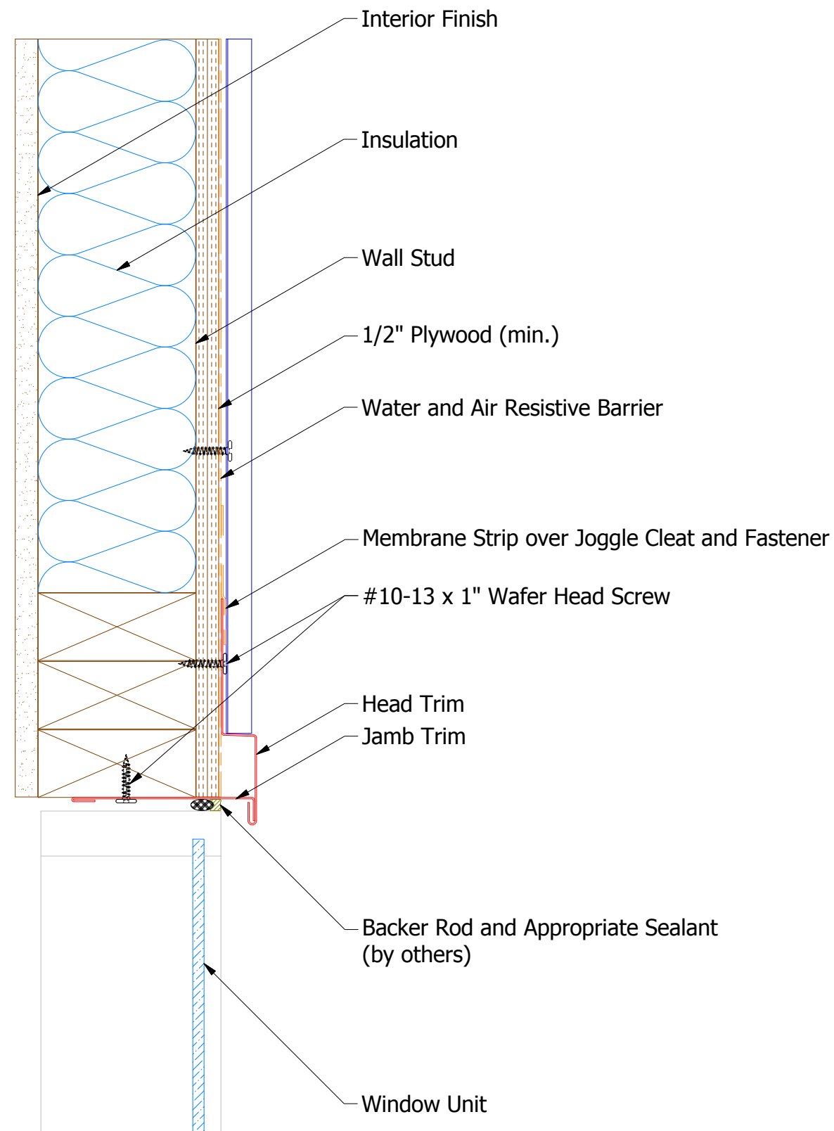
Vertical Application
