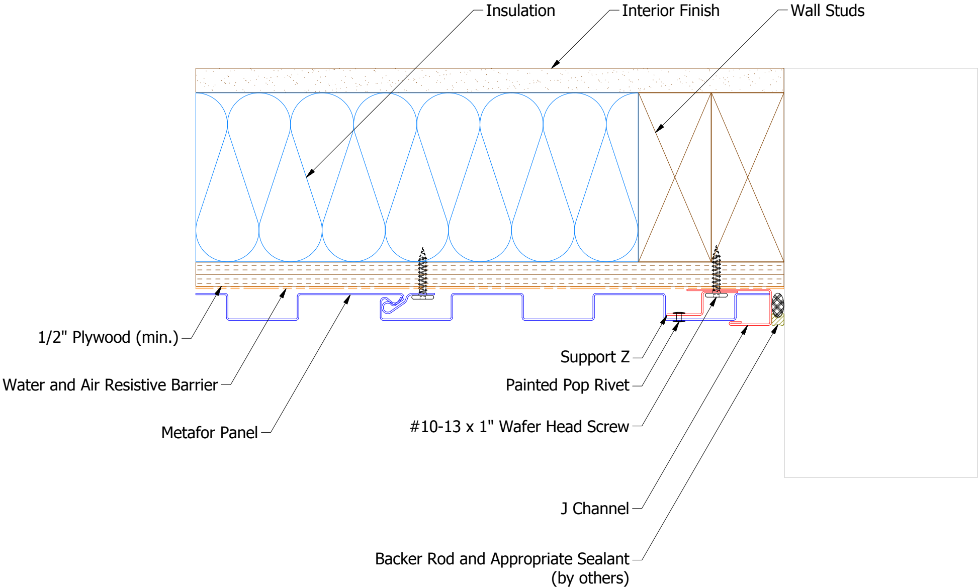
Vertical Application
