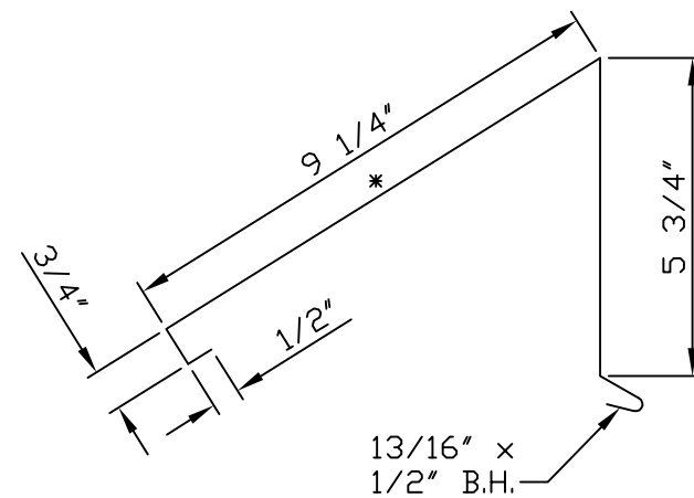
(20) - MRA364 - VENTED SHED RIDGE CAP Roof slopes 6/12+ to 9/12 Ridge splice to match ridge cap 6" long each; MDA365
