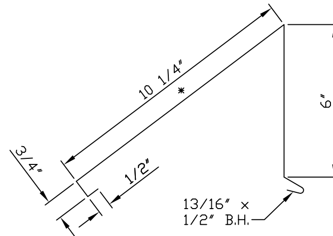
(20) - MRA366 - VENTED SHED RIDGE CAP Roof slopes 9/12+ to 12/12 Ridge splice to match ridge cap 6" long each; MDA367
