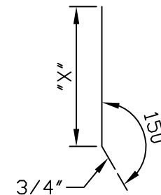
(20) - MRA364 - VENTED SHED RIDGE CAP Roof slopes 6/12+ to 9/12 Ridge splice to match ridge cap 6" long each; MDA365
