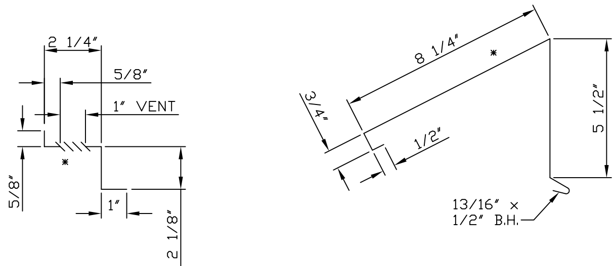
(20) - MRA362 - VENTED SHED RIDGE CAP Roof slopes 3/12+ to 6/12 Ridge splice to match ridge cap 6" long each; MDA363
