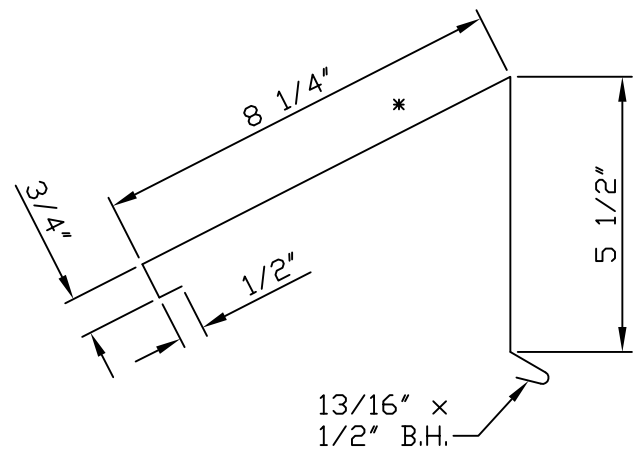
(20) - MRA362 - VENTED SHED RIDGE CAP Roof slopes 3/12+ to 6/12 Ridge splice to match ridge cap 6" long each; MDA363
