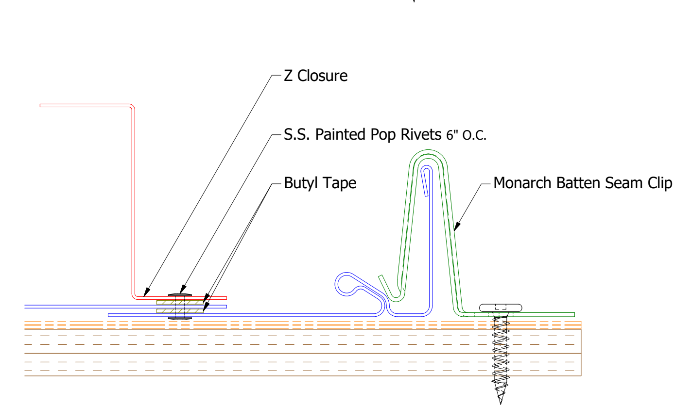
Butyl Tape Detail
