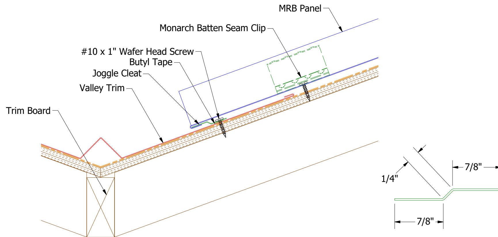
MRA975-Joggle Cleat
