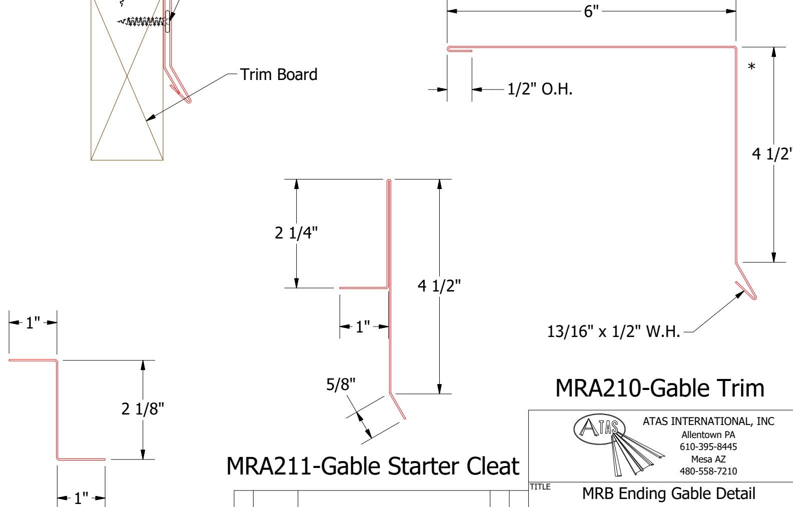
MRA910-Z Closure
