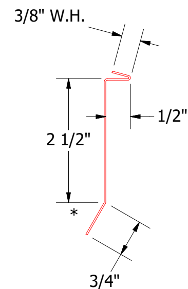
MRA980-Counterflashing
