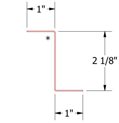
MRA910-Z Closure
