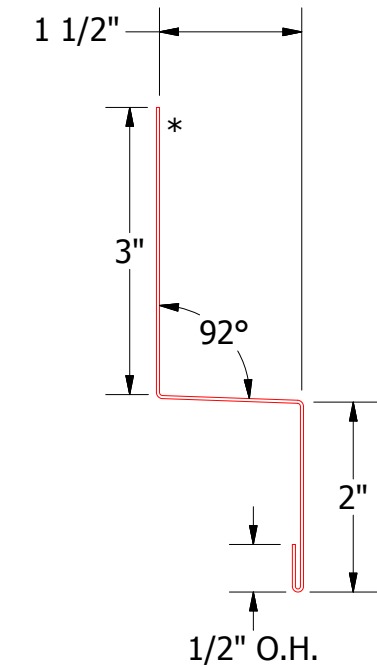
MPA550 - Head Trim
