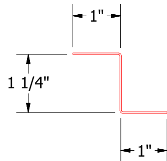
MPA681 - Support Z
