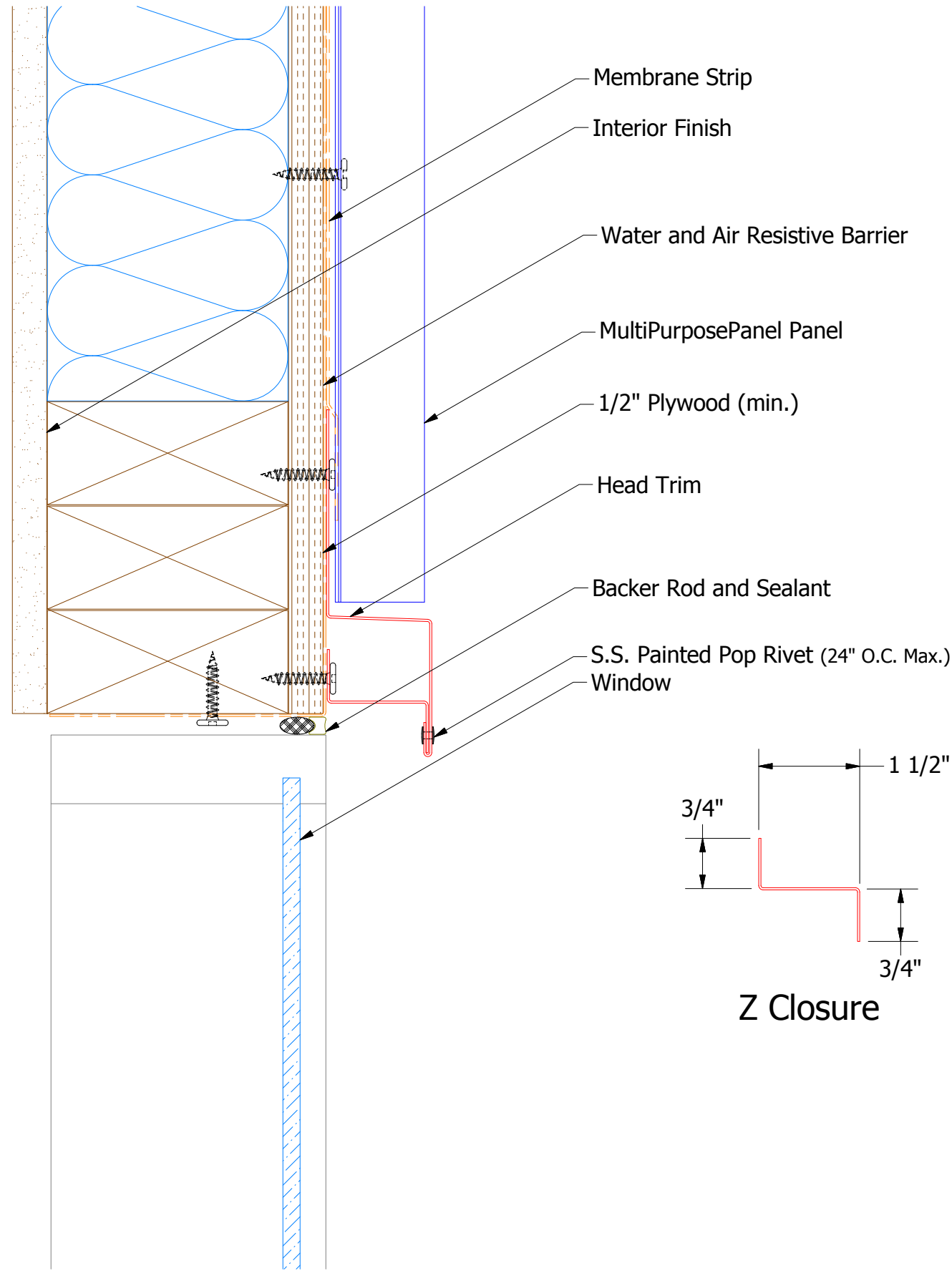
MPA550 - Head Trim
