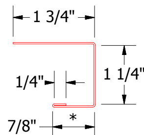
MPA138 - J Channel
