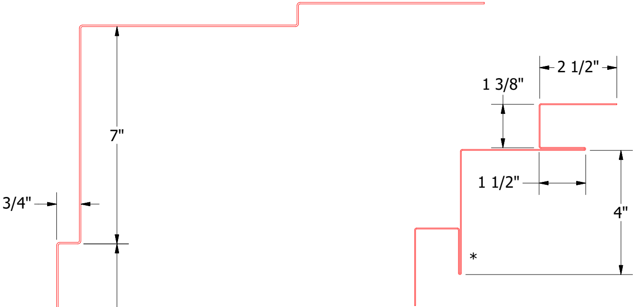
Alternate Subgirt Orientation
