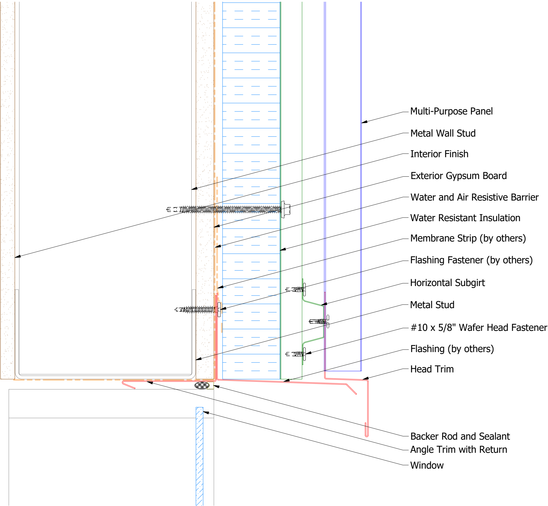
MPA550-Head Trim
