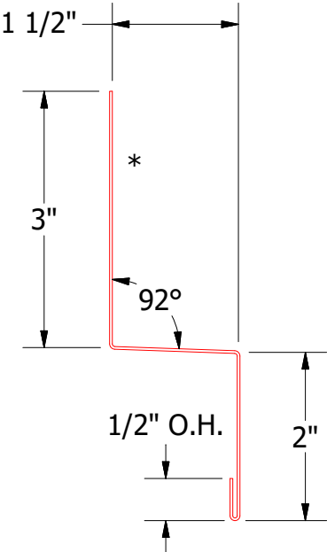
MPA550-Head Trim
