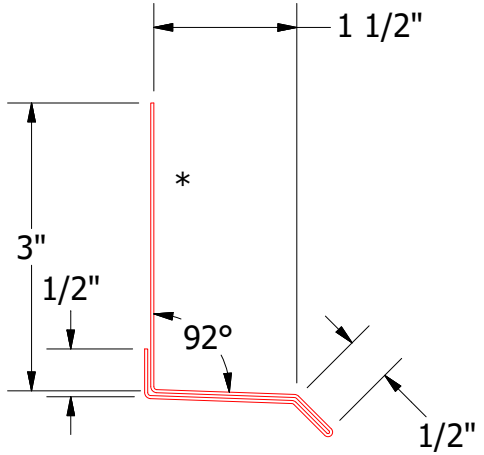
MPA661-Base Trim
