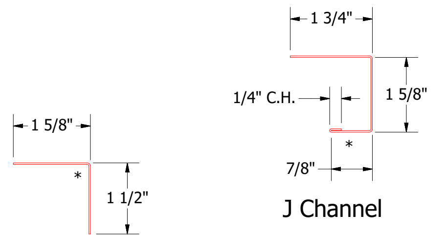
Angle Trim
