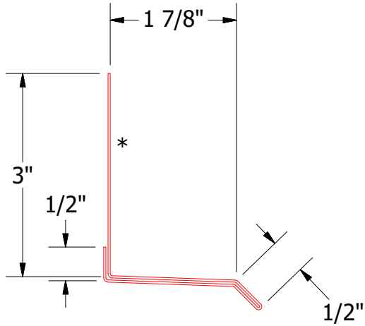
Base Trim
