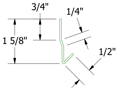
Starter Cleat
