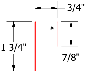
OPA270 - J Closure
