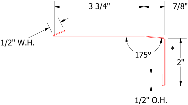
OPA670 - Window Sill Trim
