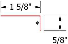
OPA680 - Angle Trim
