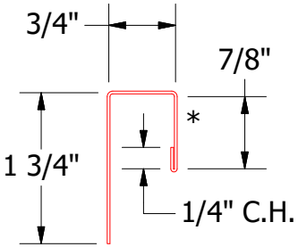
OPA034 - J Channel
