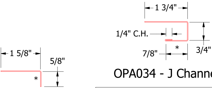
OPA680 - Angle Trim
