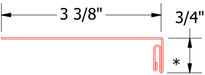
OPA039 - Snap J Base
