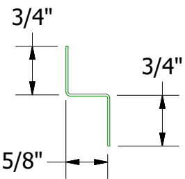
OPA681 - Support Z
