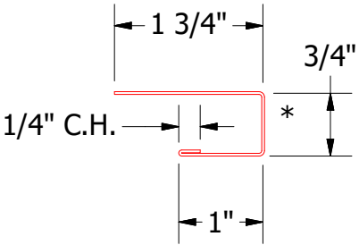
BGA034-J Channel
