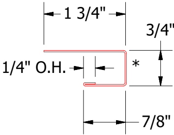
OPA034-J Channel
