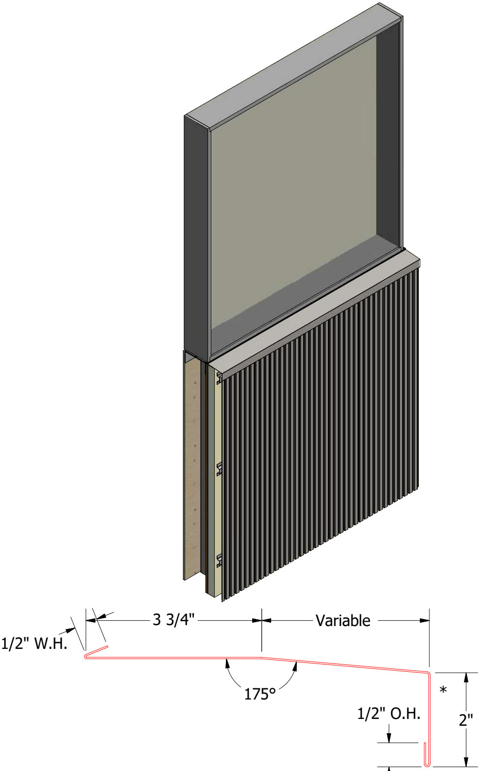
OPA670-Window Sill Trim
