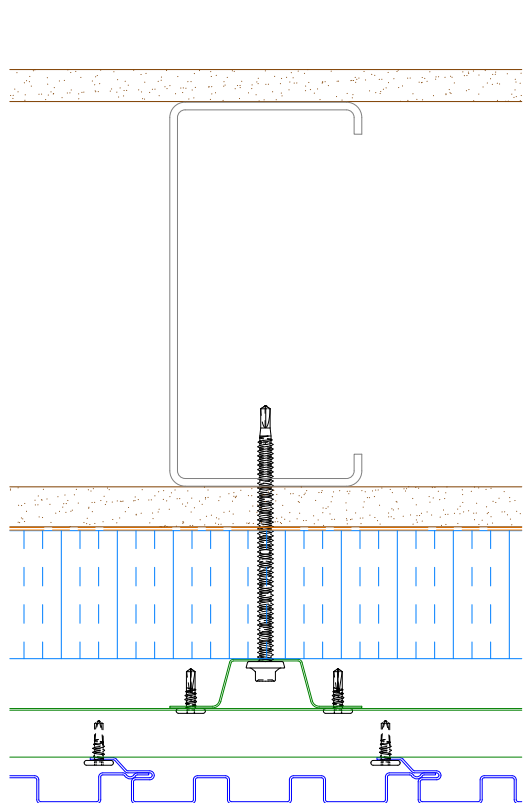
Alternate Subgirt Orientation
