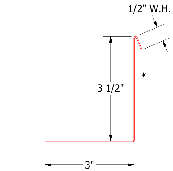
BGA683-Angle with Return
