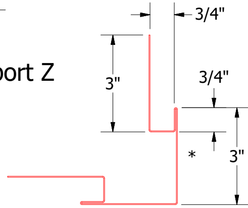
OPM602-Outside Corner Post
