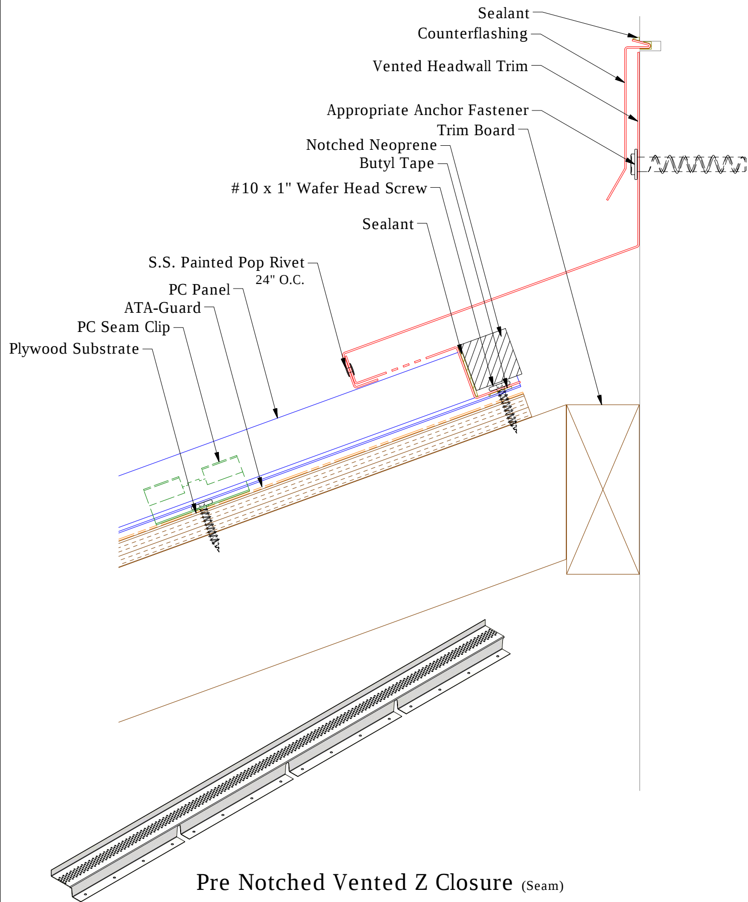
Vented Z Closure PCA911 - 1" Seam and 1" Batten D1=1 1/8" PCA913 - 2" Batten D1=2 1/8"
