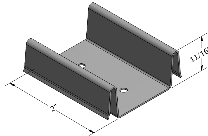
PCB900 - PC Batten Clip
