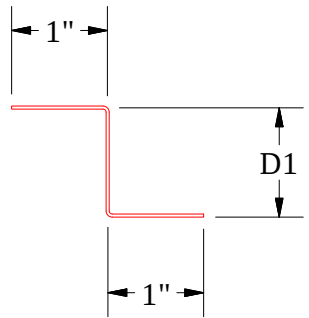
Z Closure
