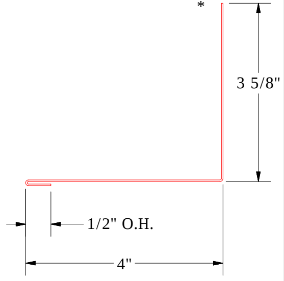
PCA410-Sidewall Trim
