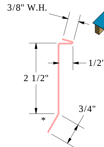
PCA980-Counterflashing
