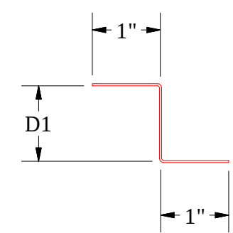
Z Closure
