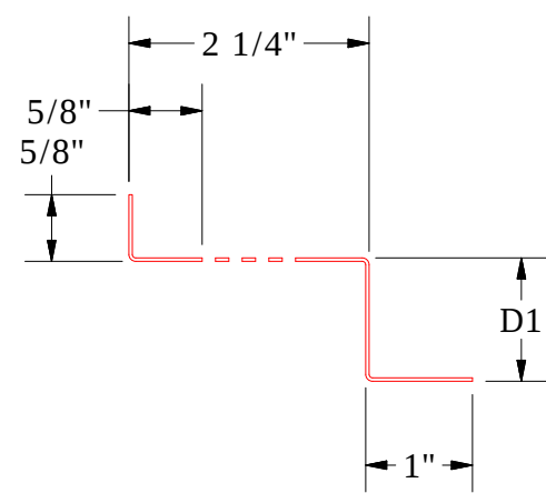
Vented Z Closure PCA911 - 1" Seam and 1" Batten D1=1 1/8" PCA913 - 2" Batten D1=2 1/8"
