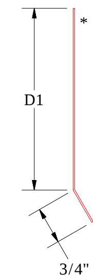
Shed Ridge Starter Cleat
