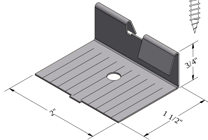
PC Seam Clip
