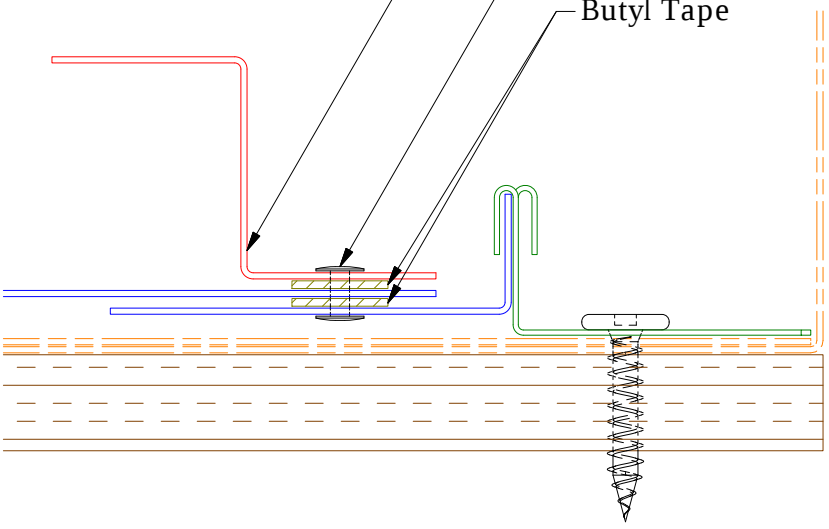
Butyl Tape Detail
