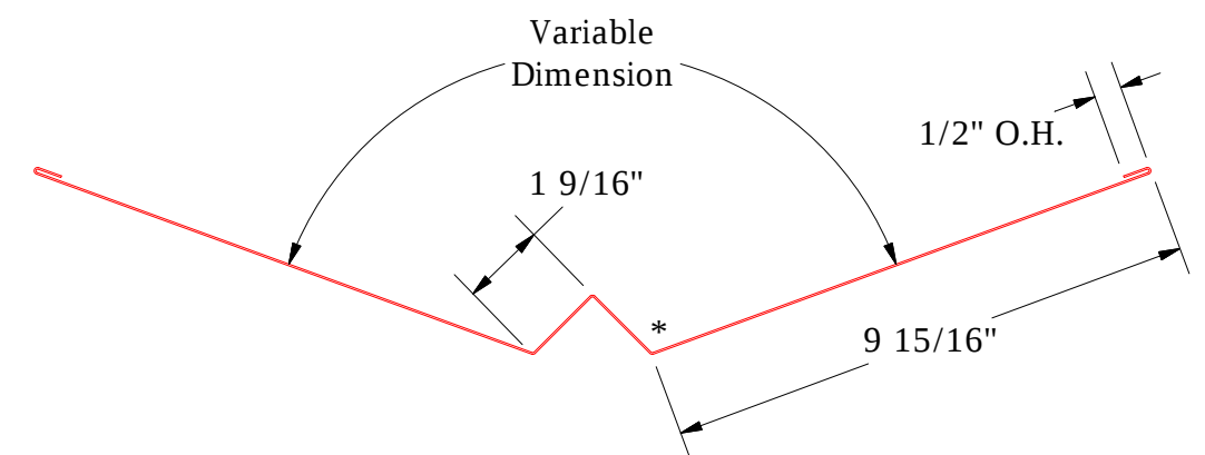
PCA800-Valley Trim
