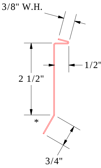
PCA980-Counterflashing
