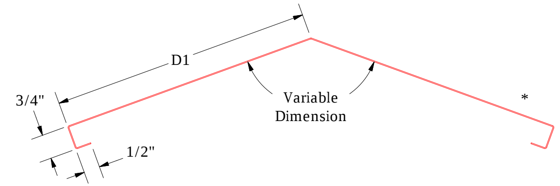
Vented Ridge Cap PCA322-3:12 to 6:12 Slope D1=7 1/4" PCA324-6:12 to 9:12 Slope D1=8 1/4" PCA326-9:12 to 12:12 Slope D1=9 1/4"
