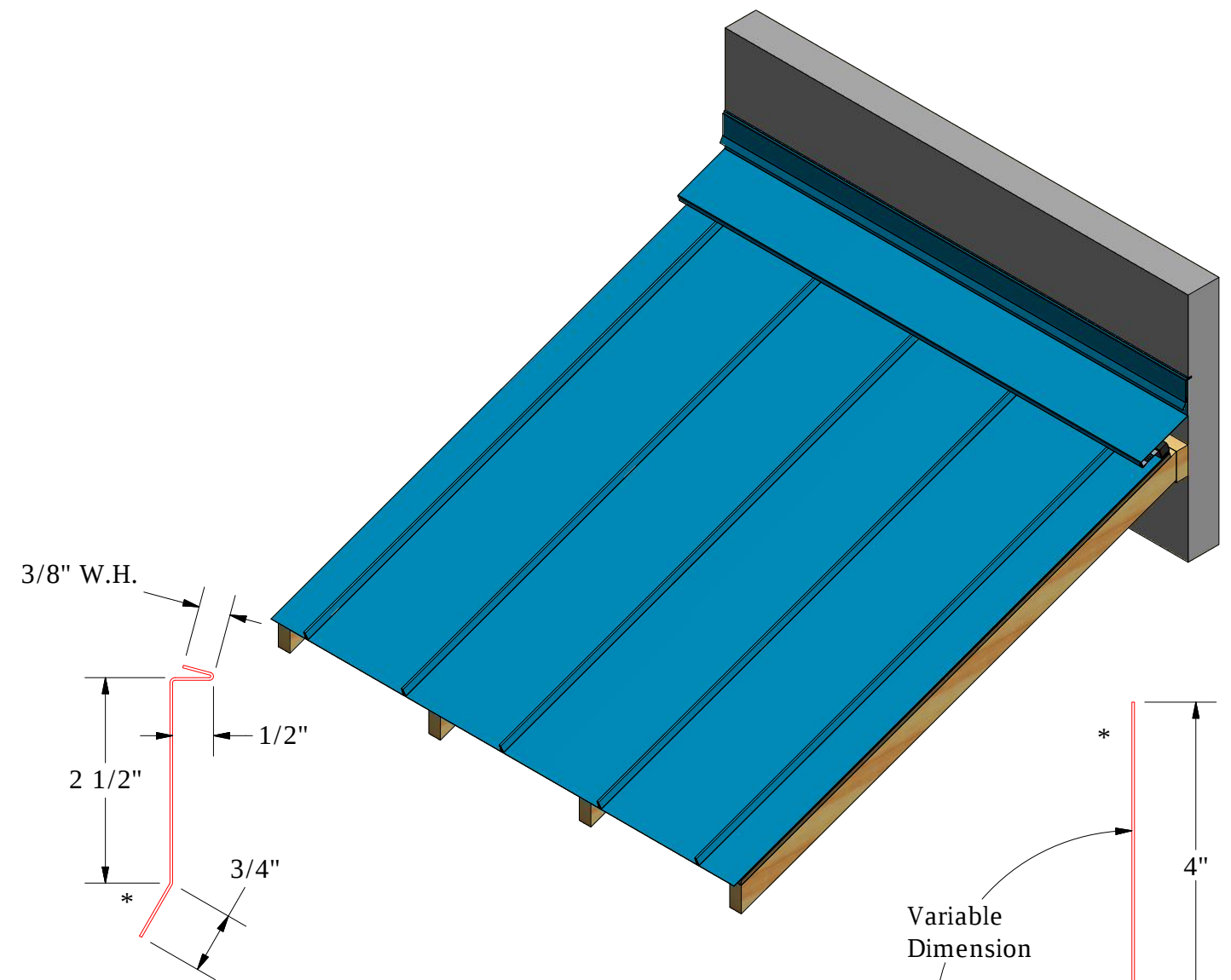
PCA980-Counterflashing
