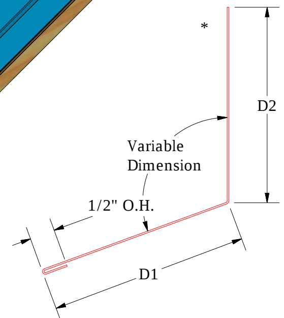
Headwall Trim
