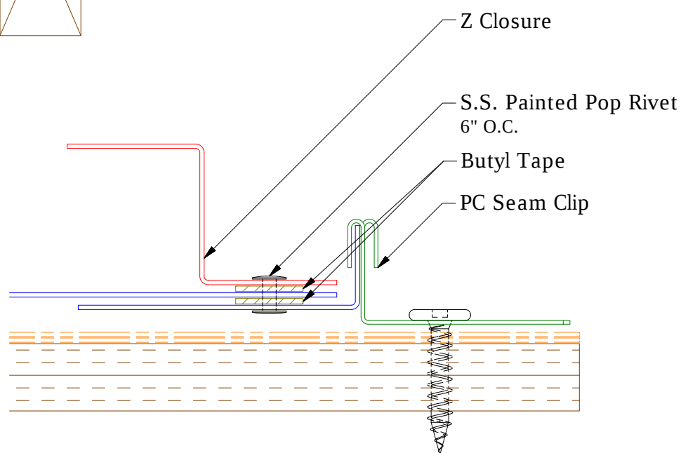
Butyl Tape Detail
