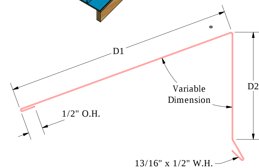
Shed Ridge Cap
