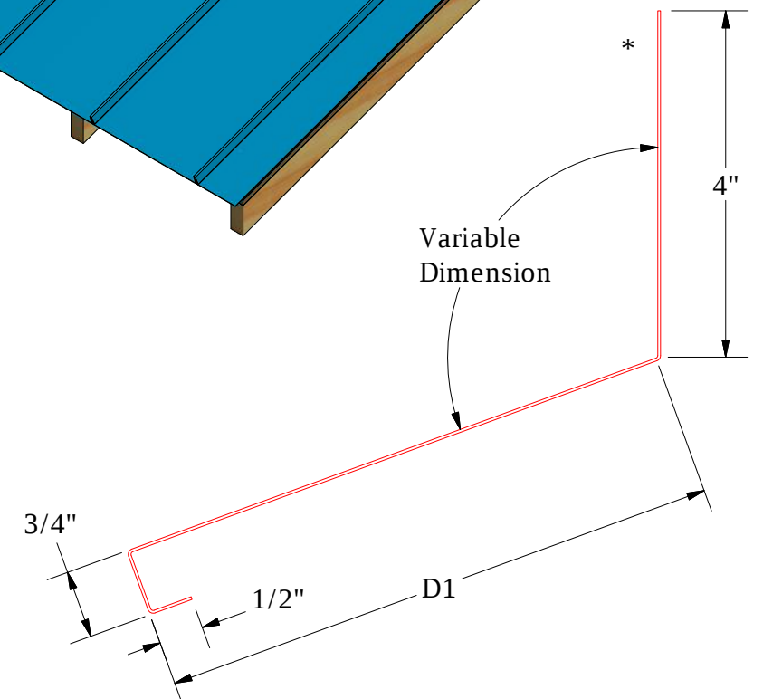
PCA510-Vented Headwall Trim
