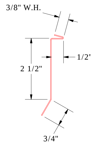
PCA980-Counterflashing
