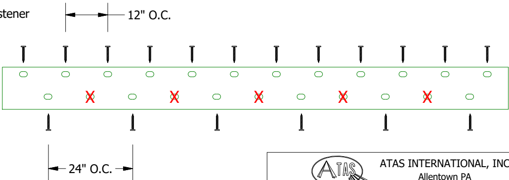
Cleat Fastener Location per ES-1 Testing
