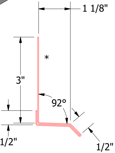
MCA661-Base Trim
