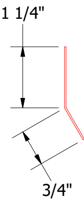
MFA995-Starter Cleat
