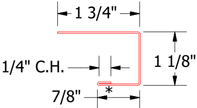
MCA118 - J Channel
