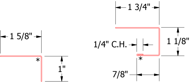
MCA680 - Angle Trim MCA118 - J Channel
