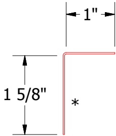
MCA680 - Angle Trim
