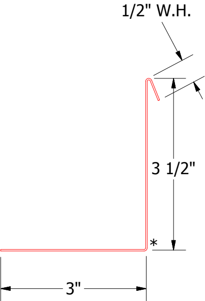
MCA683 - Angle Trim Without Return
