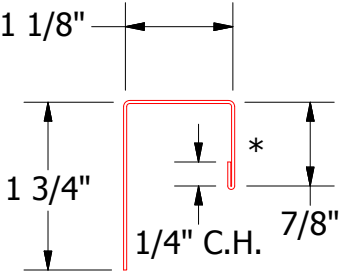
MCA118 - J Closure
