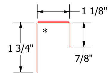
MCA270 - J Closure
