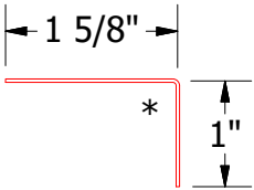
MCA680 - Angle Trim
