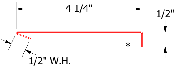
MCA690 - Head Angle Trim
