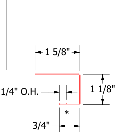
MCA118-J Channel
