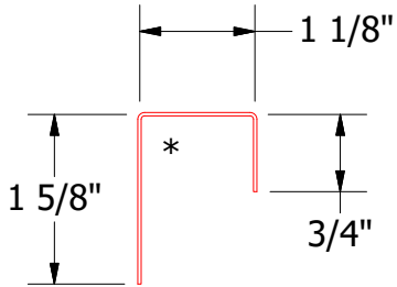
MCA270-J Closure
