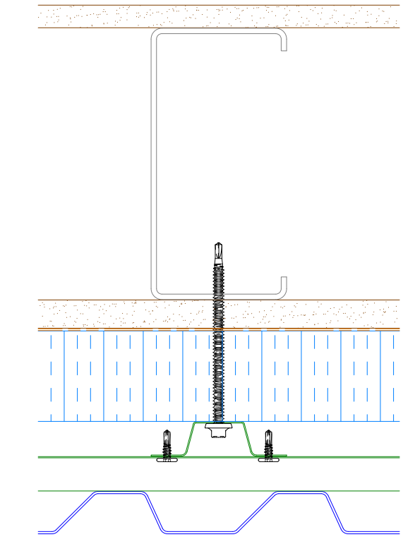
Alternate Subgirt Orientation (NTS)
