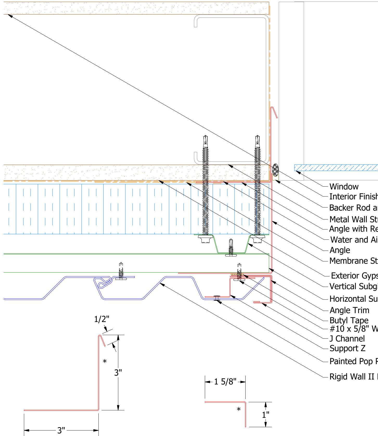
MCA680-Angle Trim
