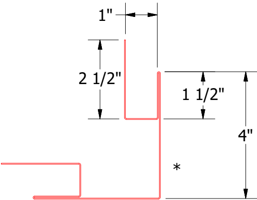
MCA602-Outside Corner Post
