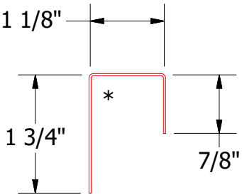
MCA118-J Channel
