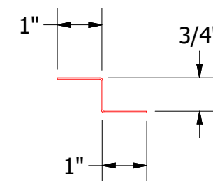
Support Z
