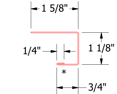
MCA118-J Channel
