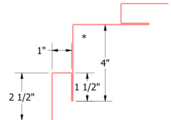
MCA601 - Inside Corner Post
