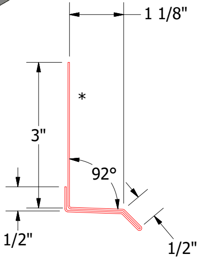
MCA661-Base Trim
