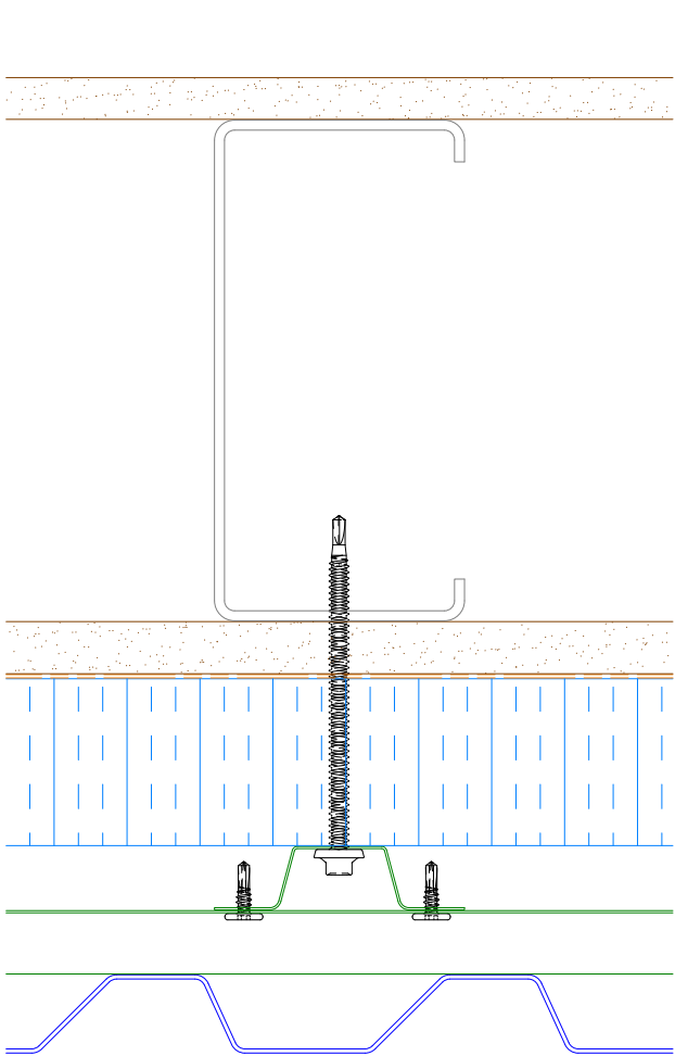
Alternate Subgirt Orientation (NTS)
