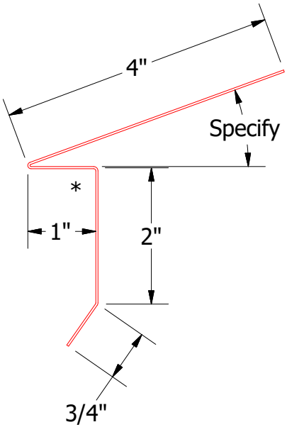
HBA113-Eave Trim
