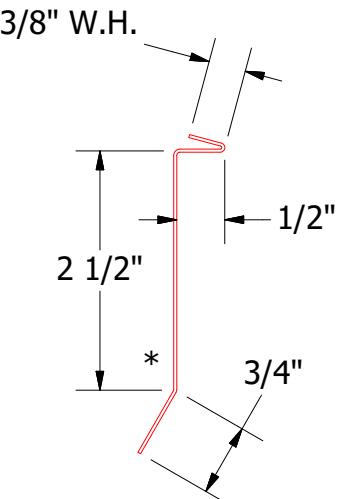
HBA980-Counterflashing
