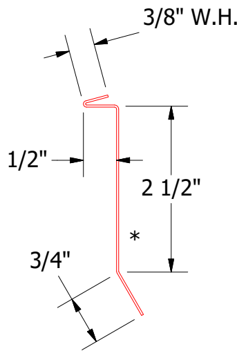
HBA980-Counterflashing
