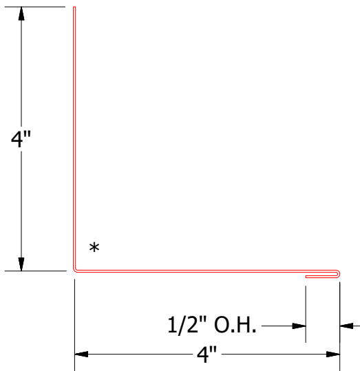
HBA410-Sidewall Trim
