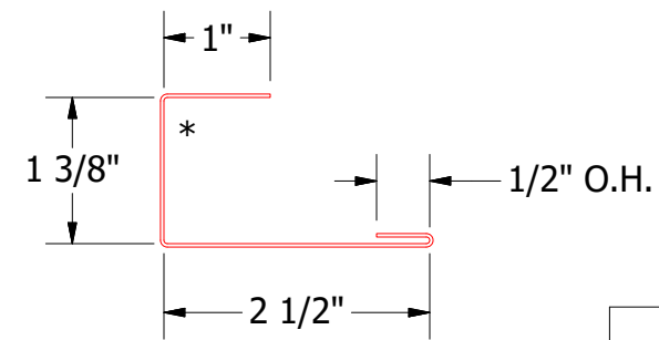
HBA200-Channel Trim
