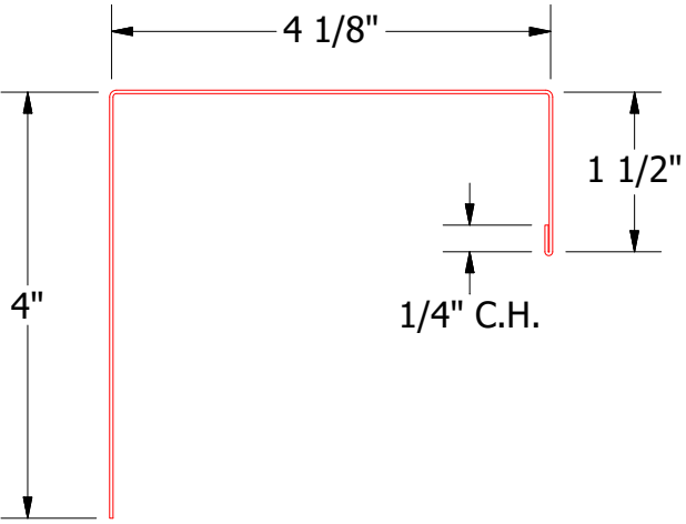
J Channel
