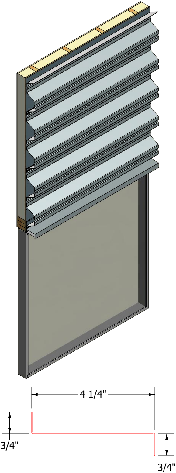
Z Closure
