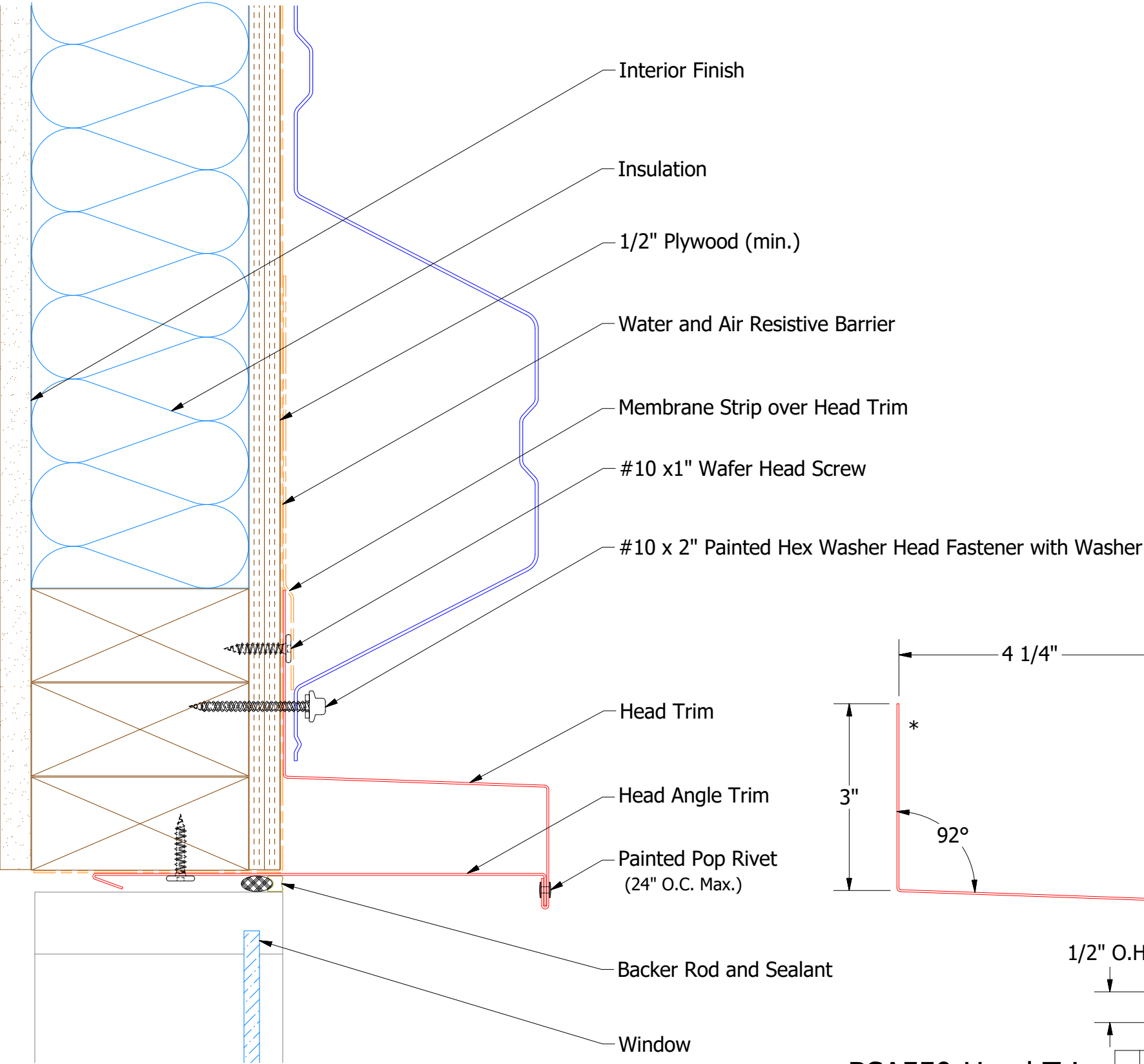
BSA550-Head Trim
