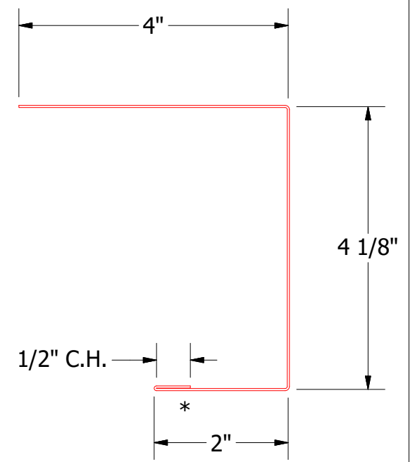
BSA140-J Channel
