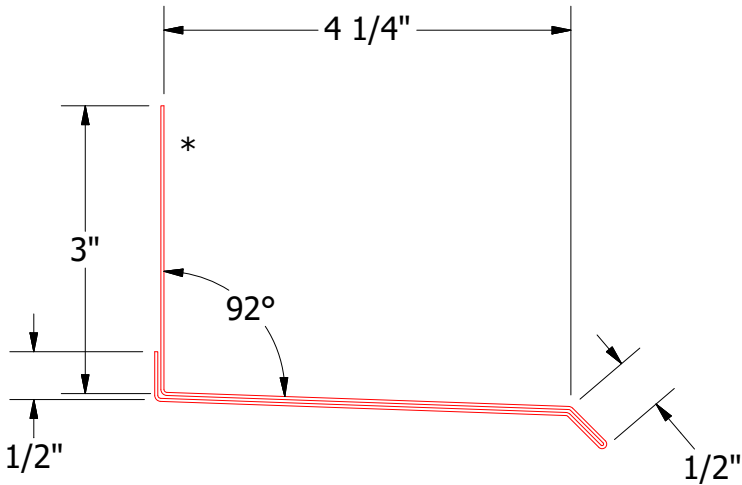
BSA661-Base Trim
