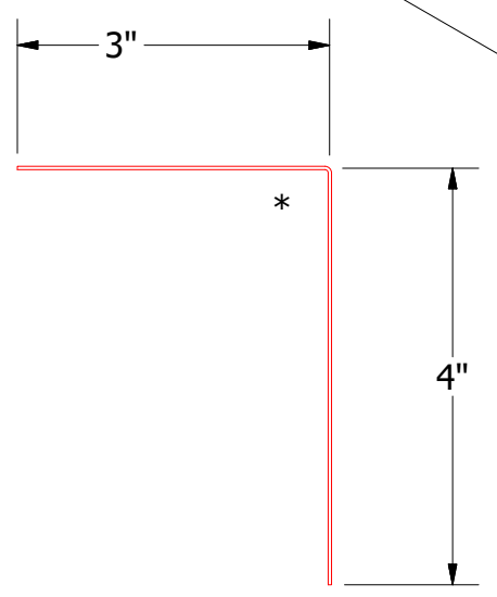
BSA680-Angle Trim
