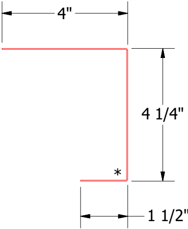
J Closure
