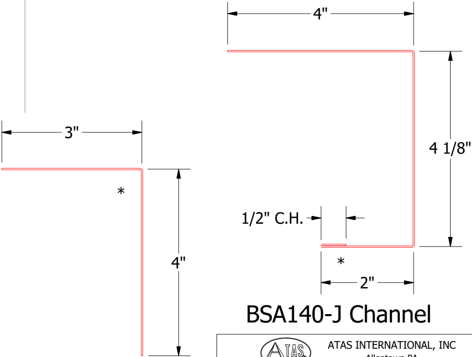
BSA680-Angle Trim
