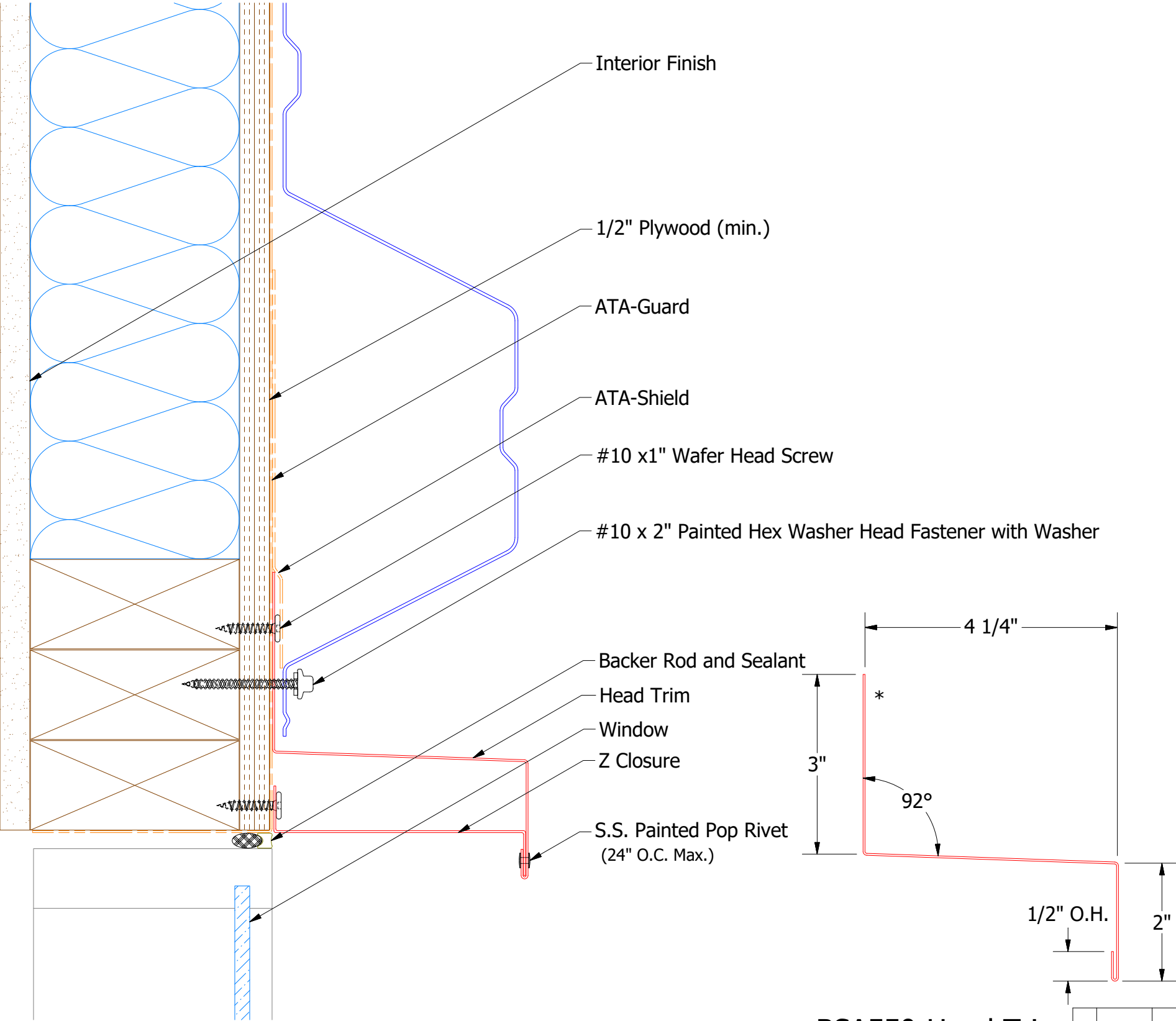
BSA550-Head Trim
