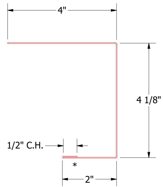
BSA140-J Channel
