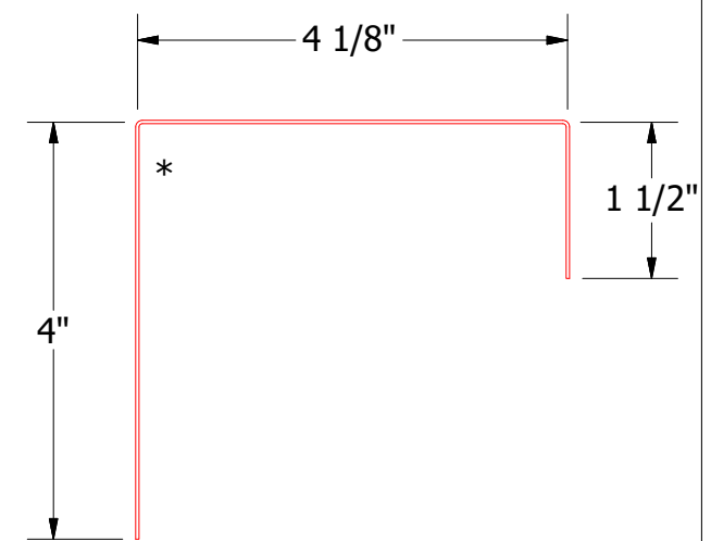
BSA270-J Closure
