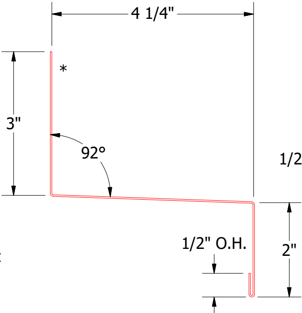
BSA550-Head Trim
