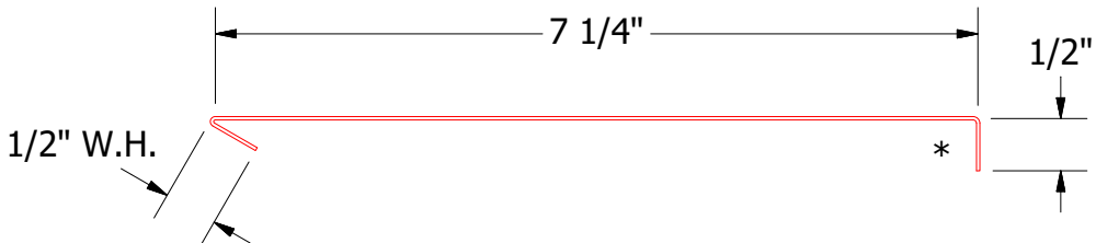
BSA690-Head Angle Trim
