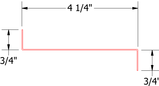
Z Closure
