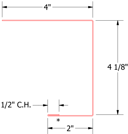
BSA140 - J Channel
