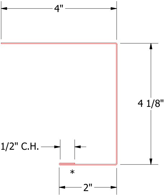
BSA140-J Channel
