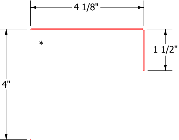
BSA270-J Closure
