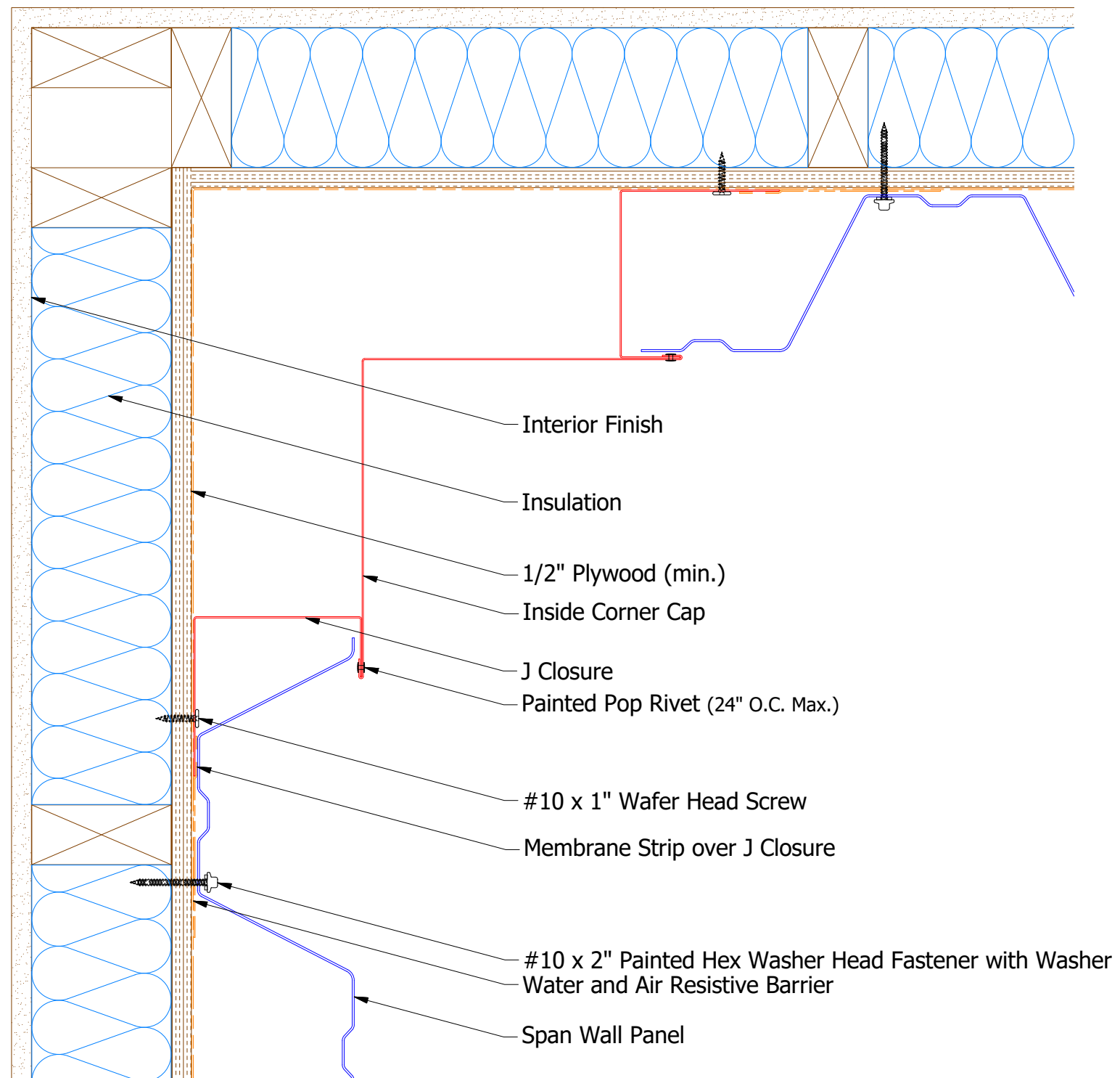
BSA270-J Closure
