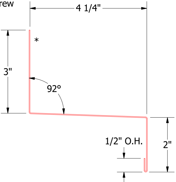
BSA550-Head Trim
