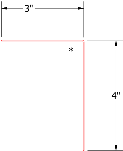
BSA680-Angle Trim
