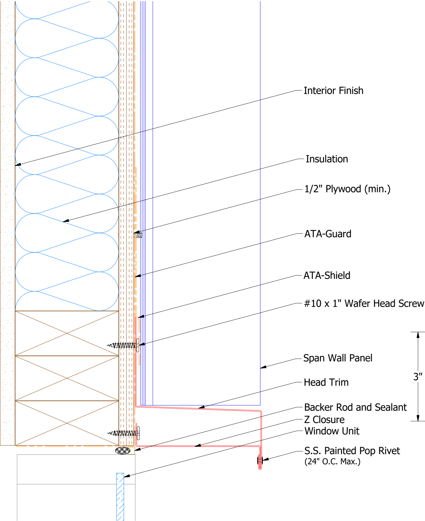
BSA550-Head Trim
