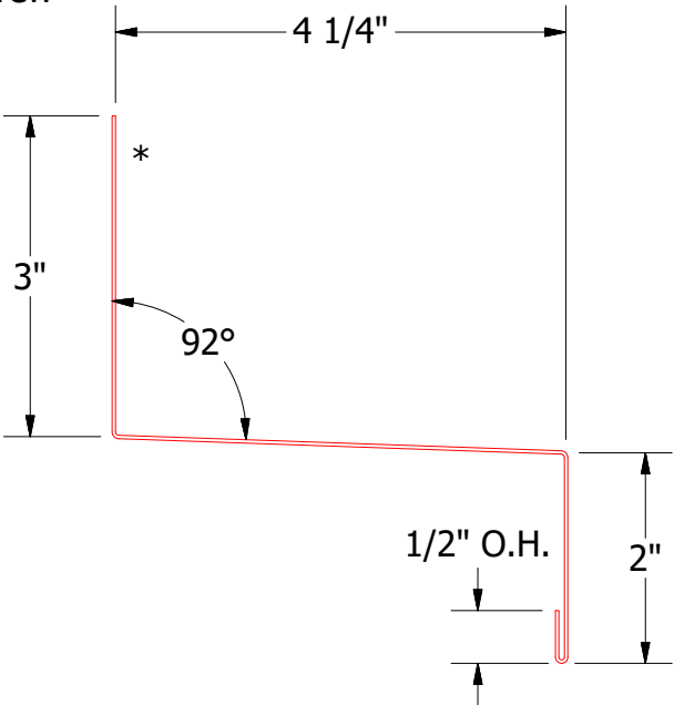
BSA550-Head Trim
