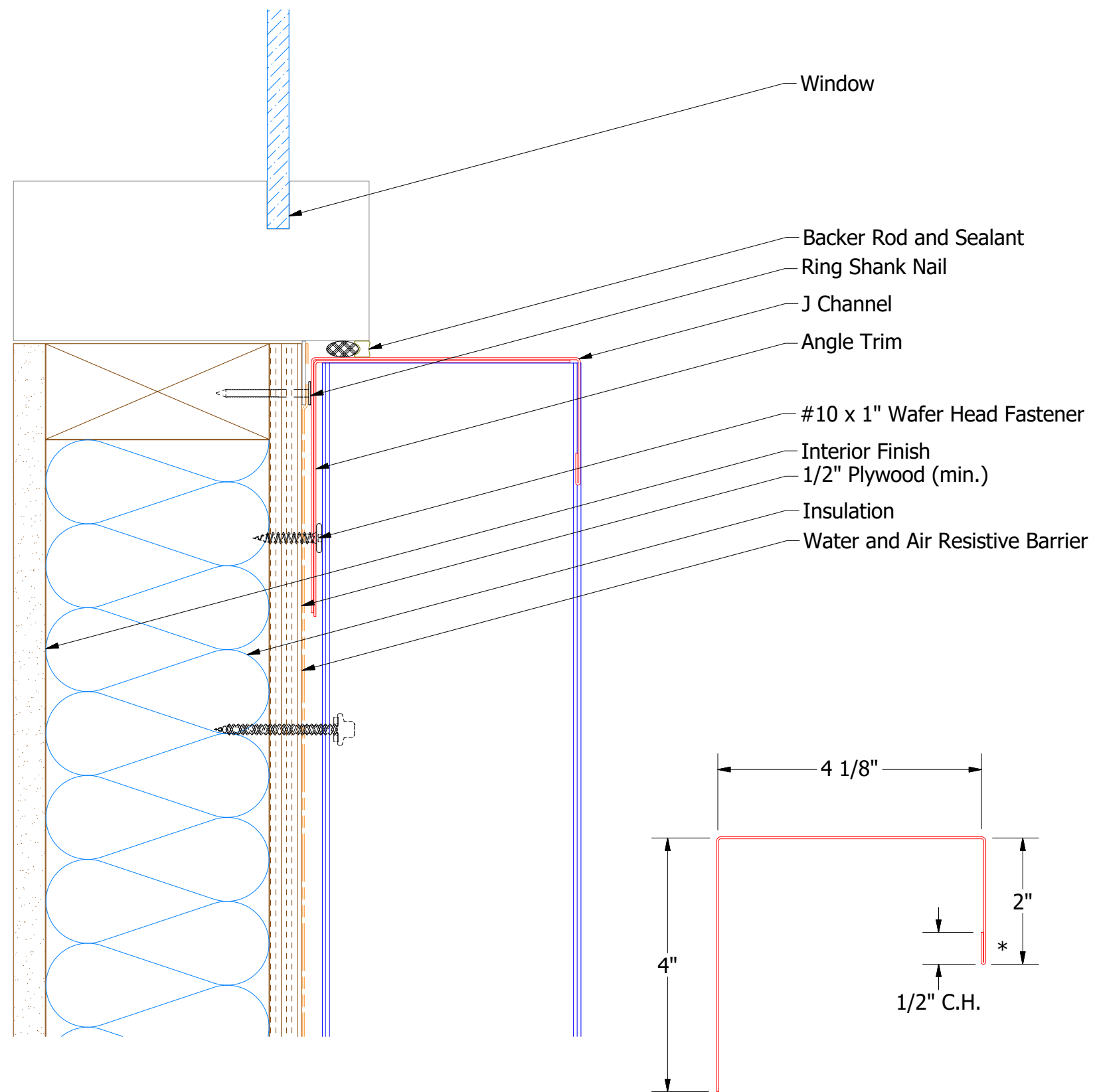
BSA140 - J Channel
