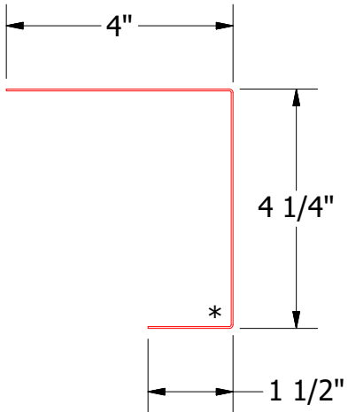
J Closure
