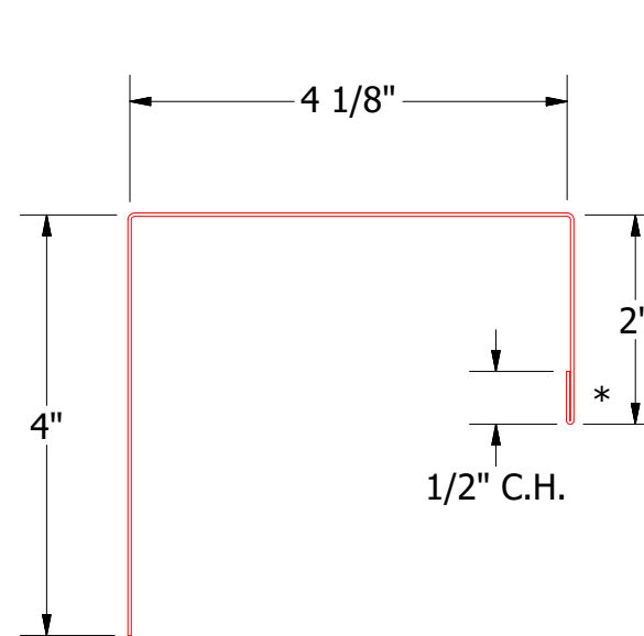
BSA140 - J Channel
