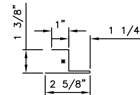
HSA910 POCKETED 'Z' CLOSURE
