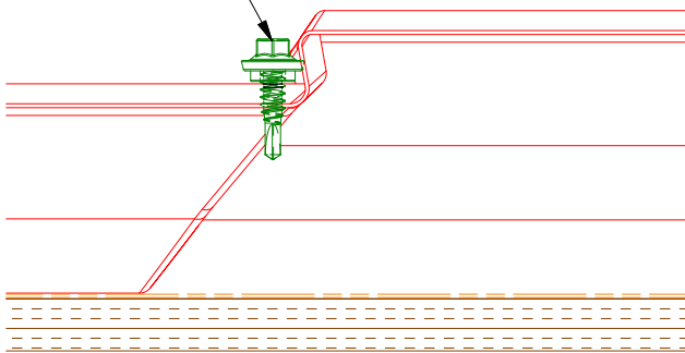
Fastener at Panel Lap
