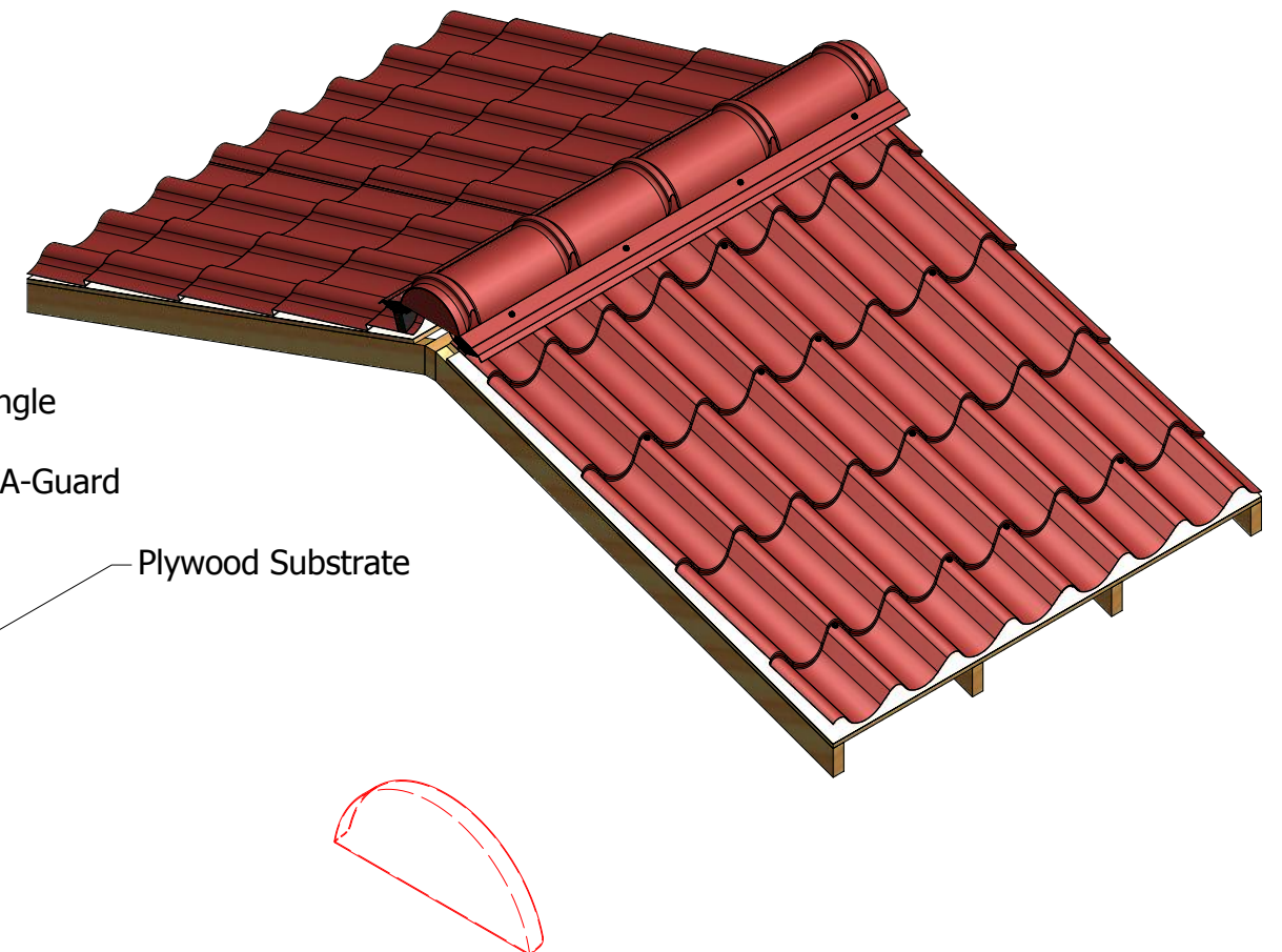
SCA375-Hip/Ridge Cap End Plug
