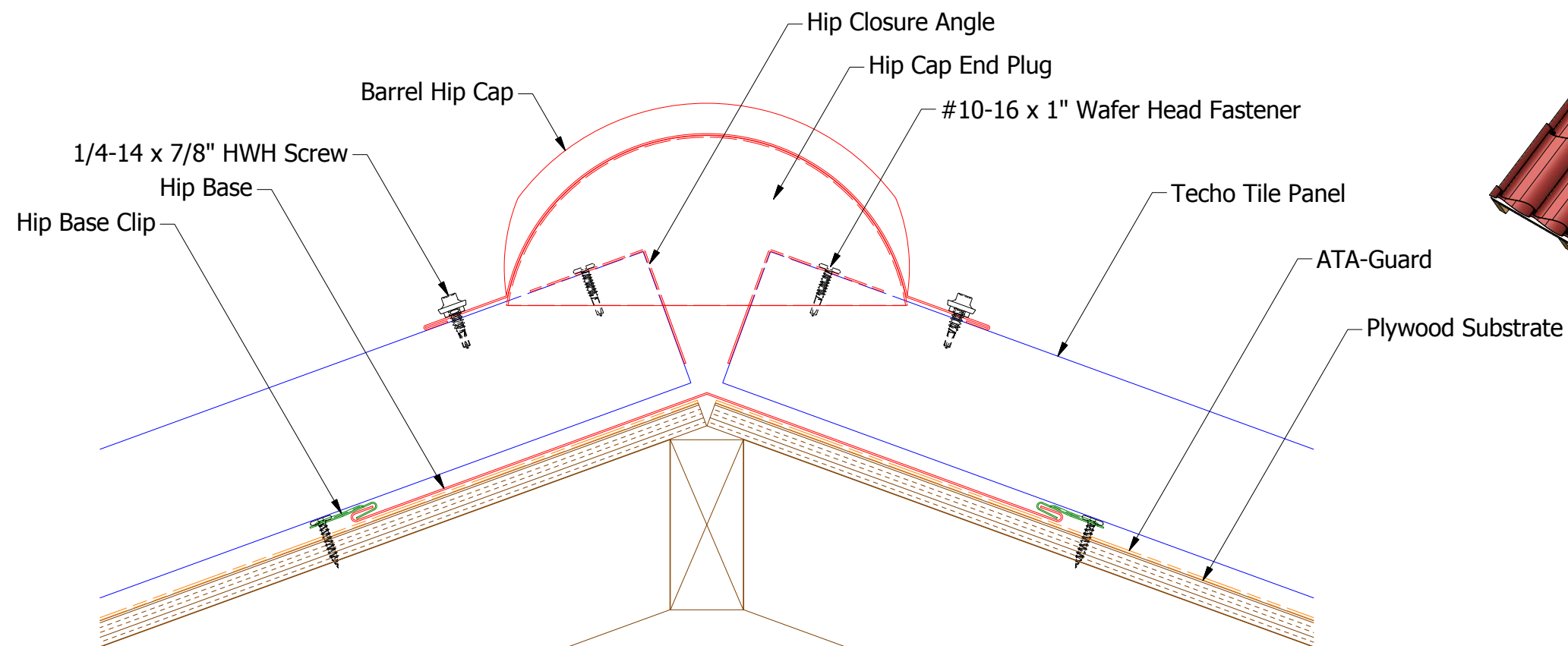
SCA375-Hip/Ridge Cap End Plug
