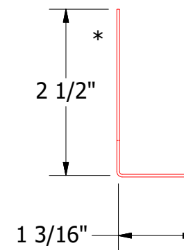
Vented Bottom Closure Angle
