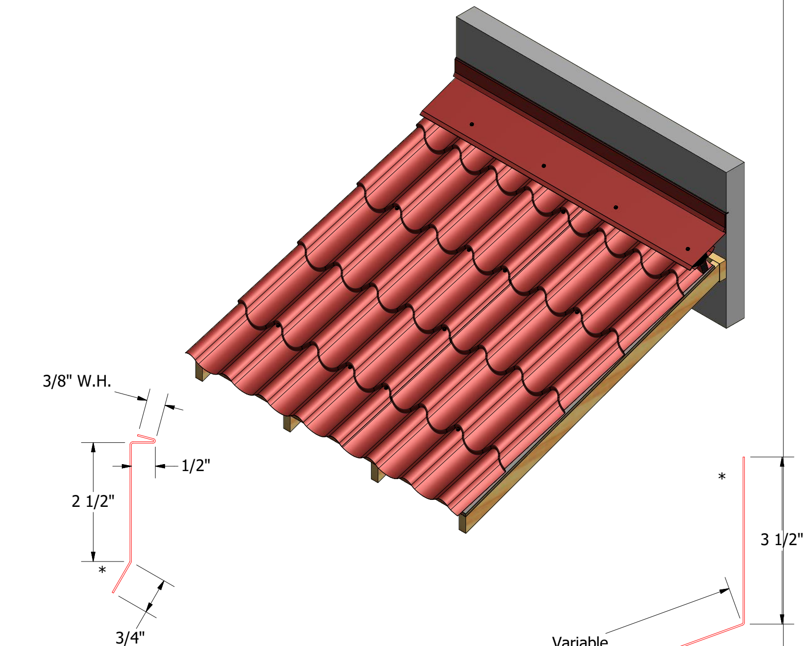
SCA980-Counterflashing
