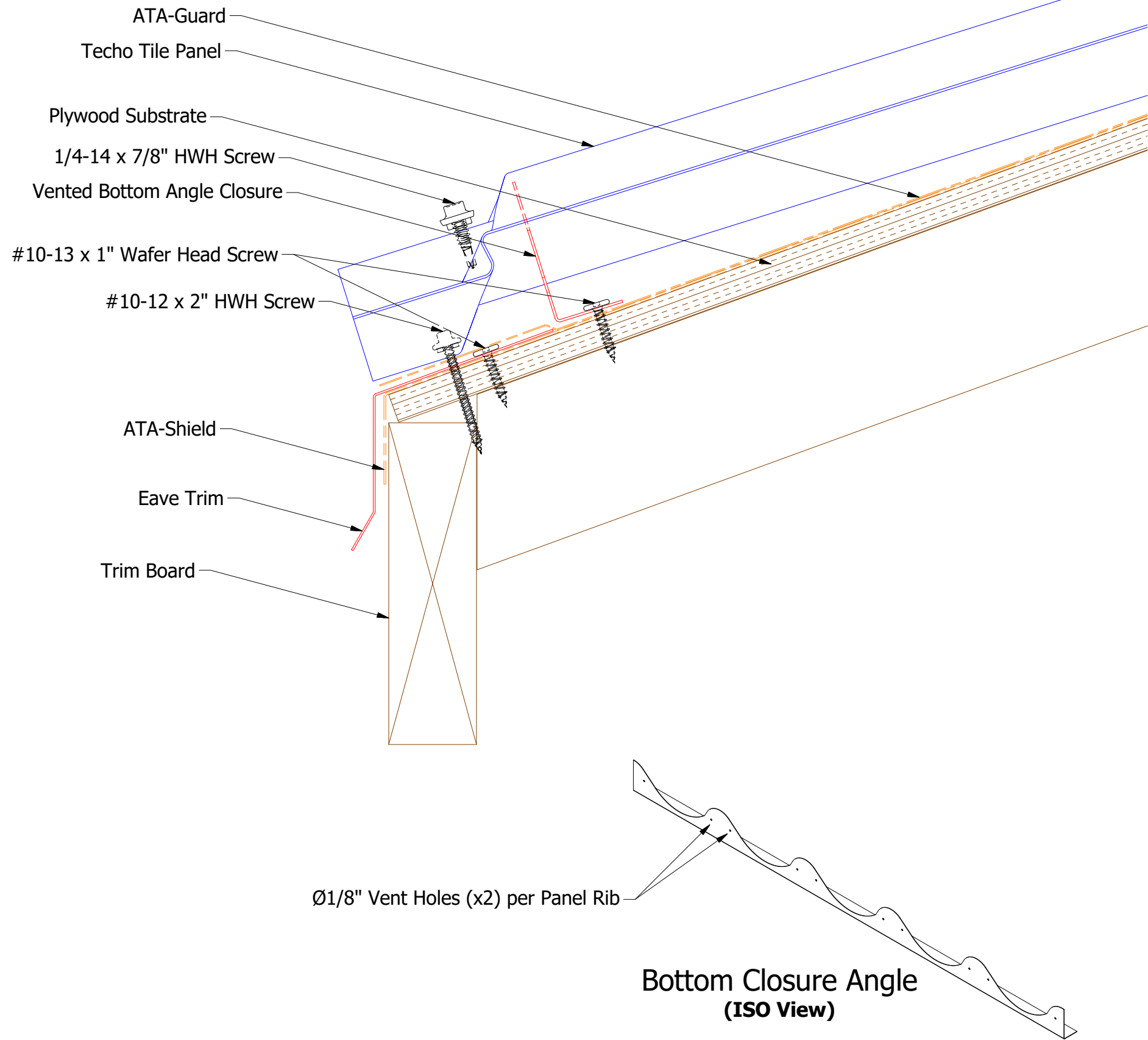
Vented Bottom Closure Angle
