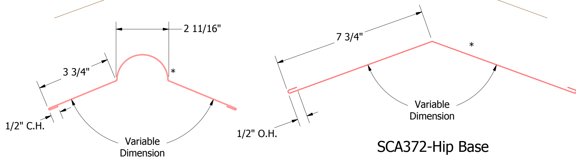
SCA303-Barrel Hip Cap (Optional)
