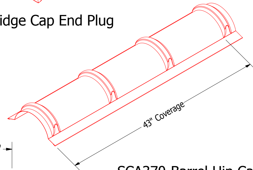
SCA370-Barrel Hip Cap (Standard)
