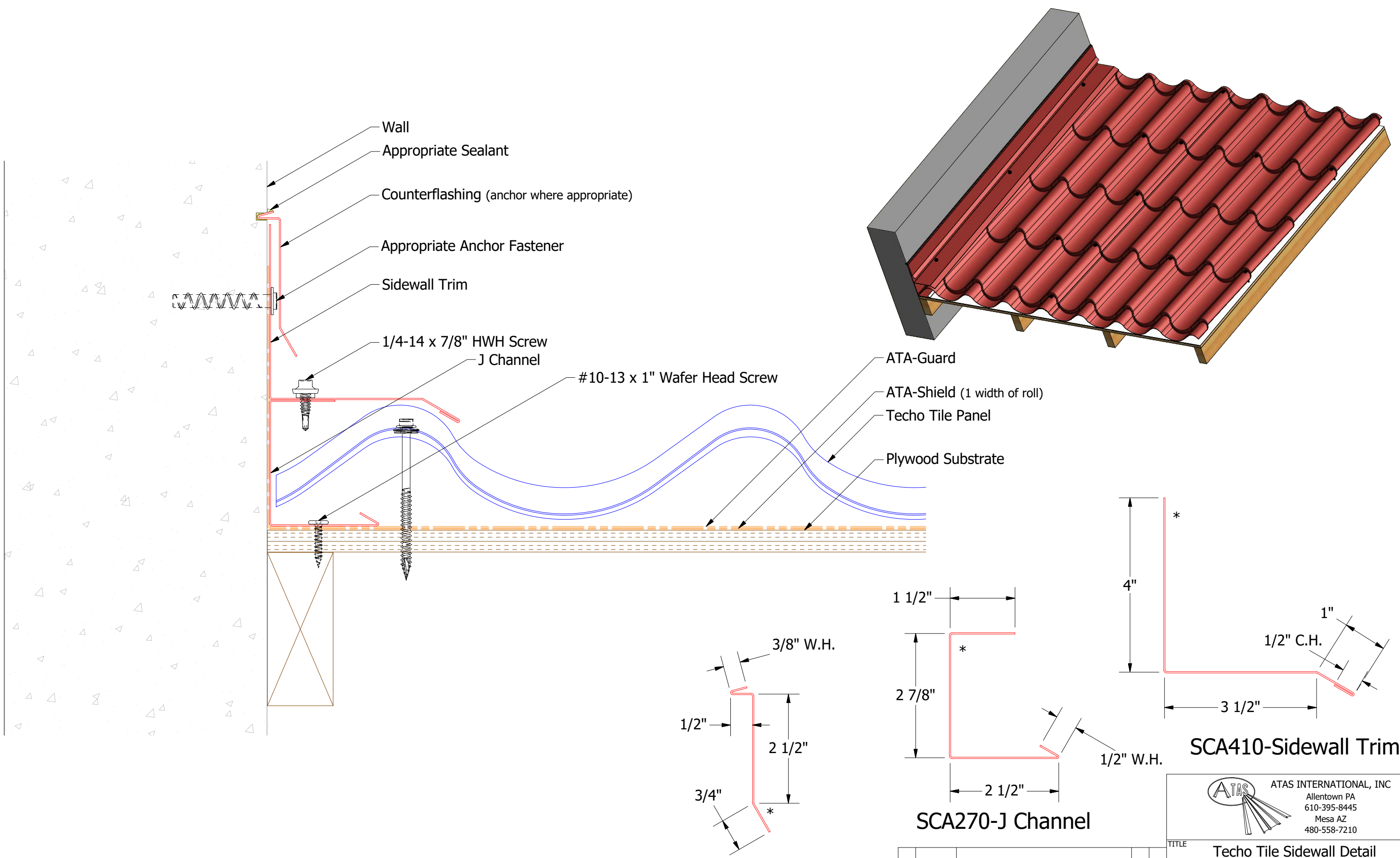
SCA980-Counterflashing
