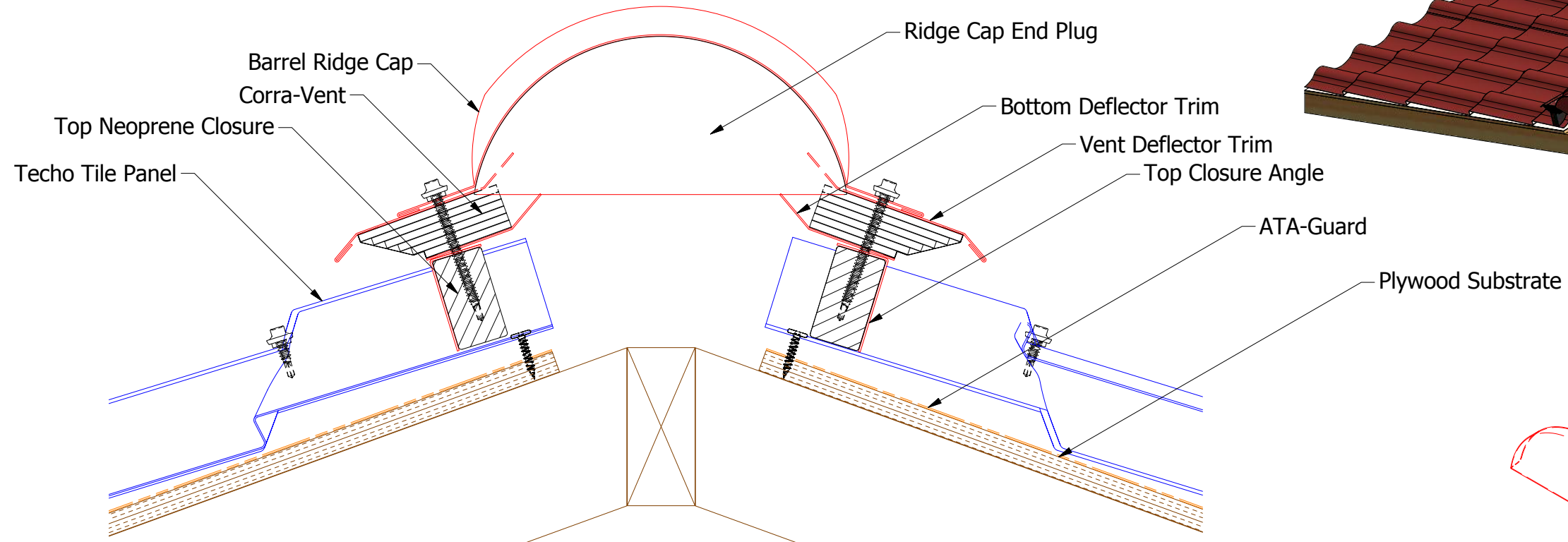
SCA375-Hip/Ridge Cap End Plug
