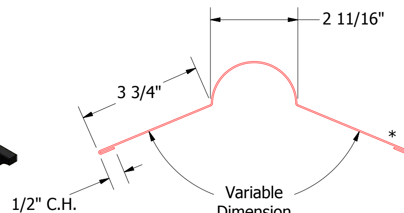
SCA303-Barrel Hip Cap (Optional)
