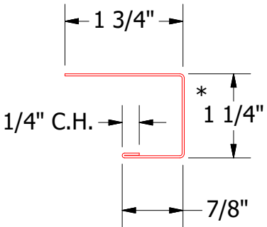
VSA118 - J Channel
