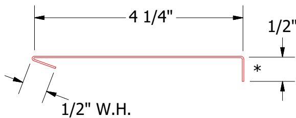
VSA690 - Head Angle Trim
