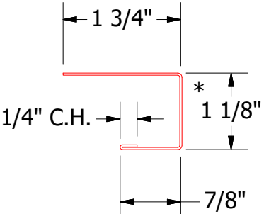
VSA118 - J Channel
