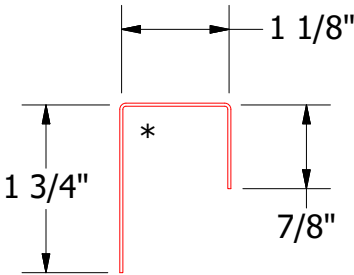
VSA270 - J Closure
