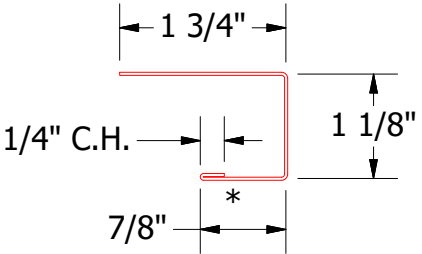
VSA118 - J Channel
