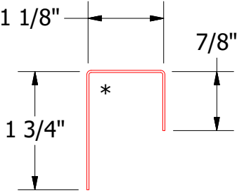
VSA270 - J Closure
