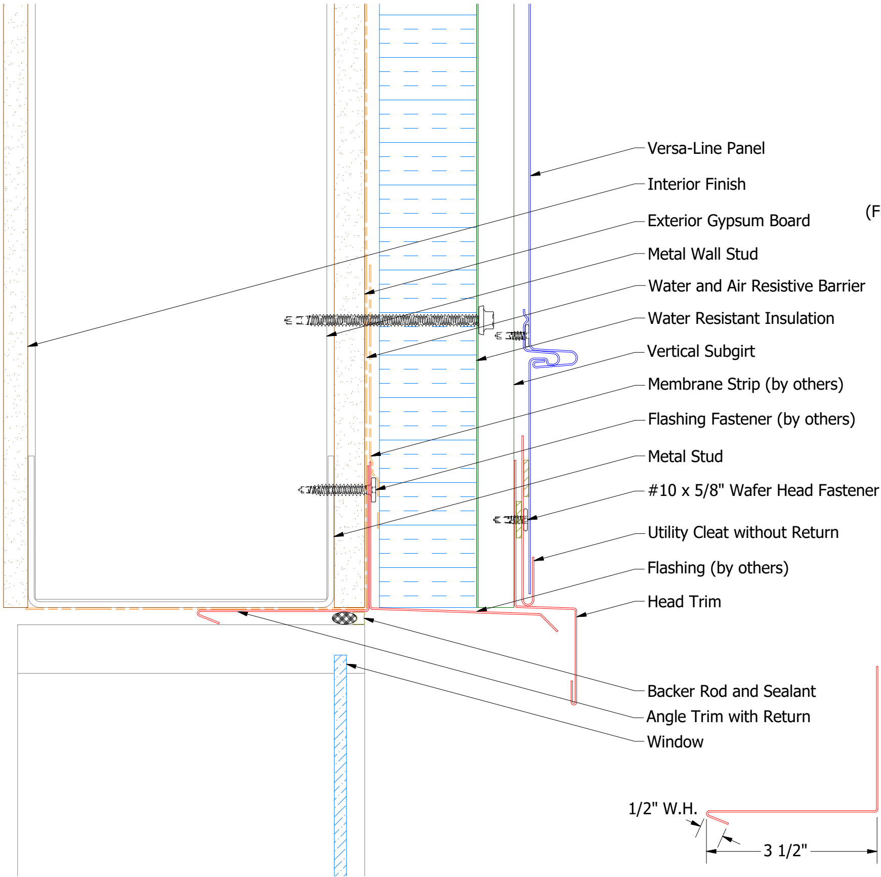
VSA683-Angle Trim with Return
