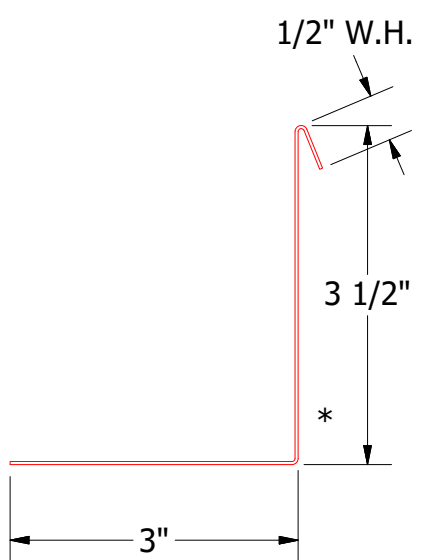
VSA683-Angle Trim with Return
