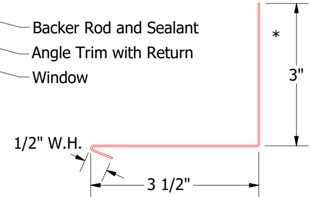
VSA683-Angle Trim with Return
