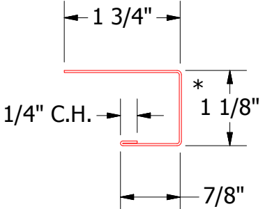
VSA118 - J Channel
