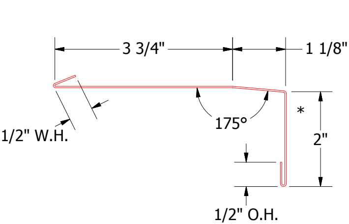
VSA670 - Window Sill Trim
