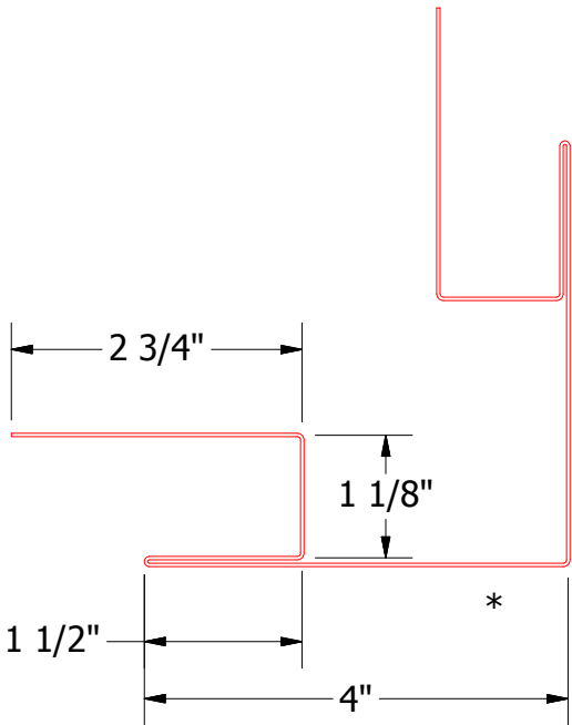
VSA602 - Outside Corner Post
