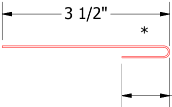
VSA962 - Utility Cleat without Return
