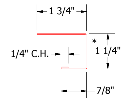
VSA118 - J Channel
