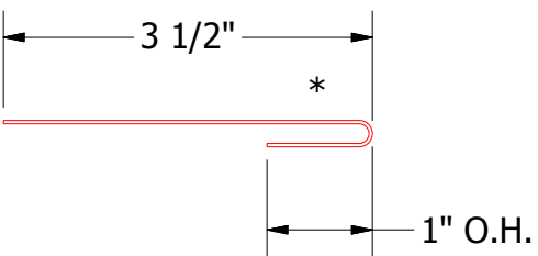
VSA962 - Utility Cleat without Return
