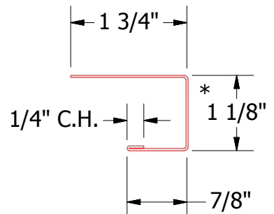
VSA118 - J Channel
