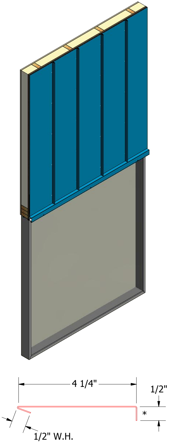
VSA690 - Head Angle Trim
