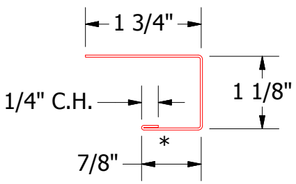
VSA118 - J Channel
