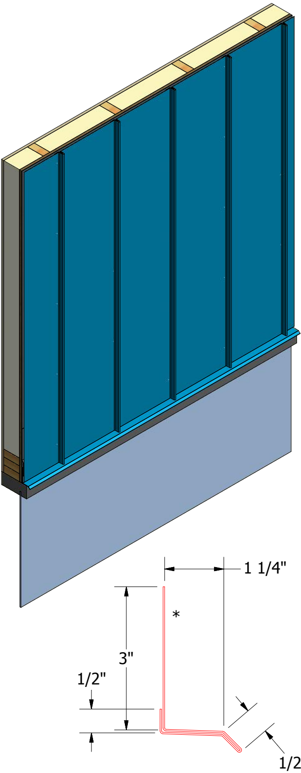
VSA661 - Base Trim - Standard
