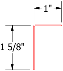
VSA280 - Angle Trim
