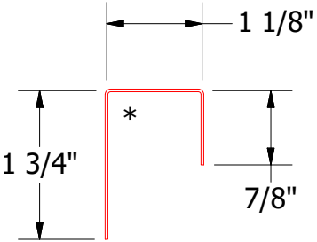
VSA270 - J Closure
