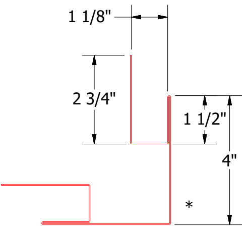
VSA602-Outside Corner Post
