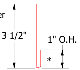
VSA962-Utility Cleat without Return
