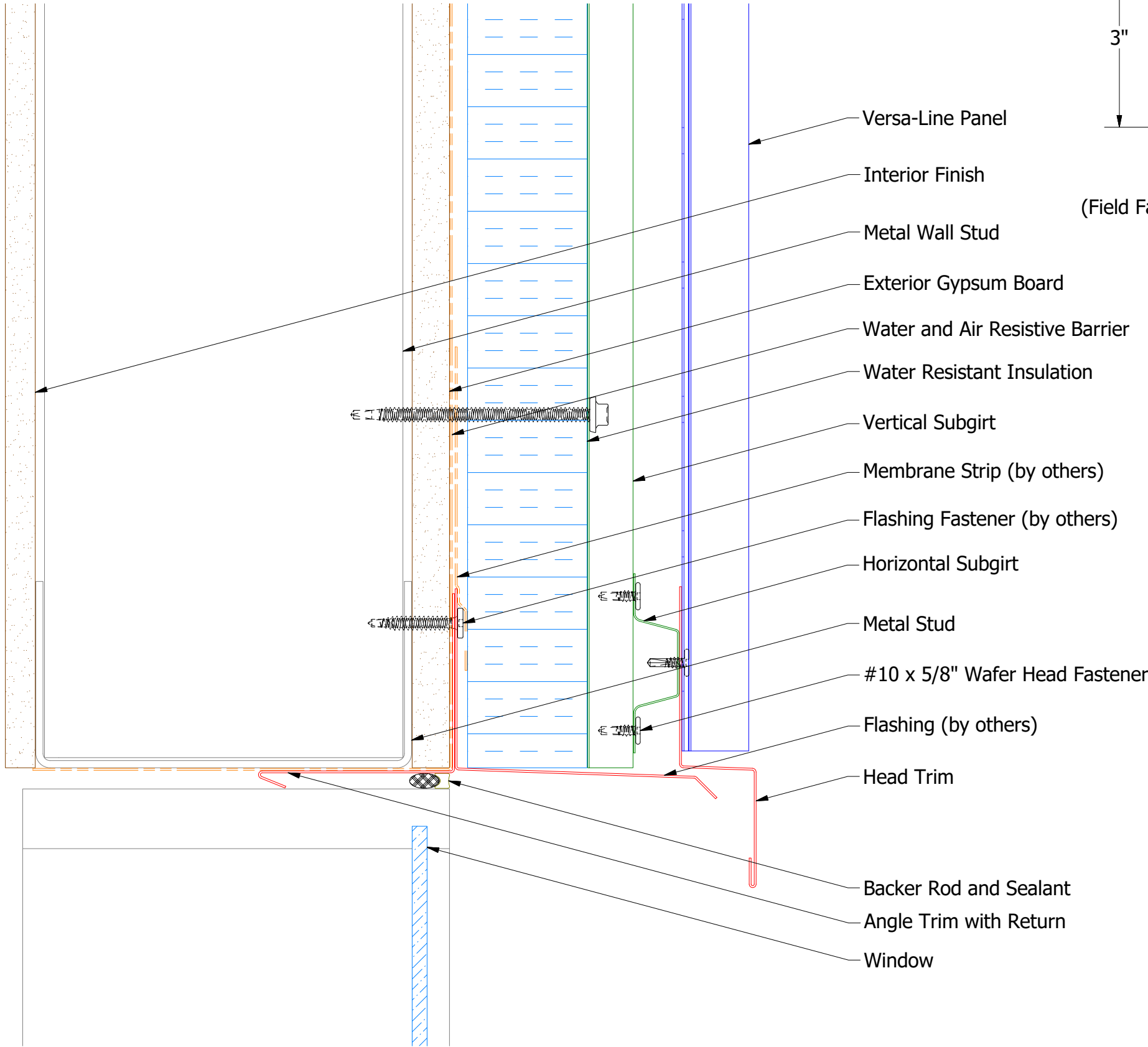
VSA550-Head Trim
