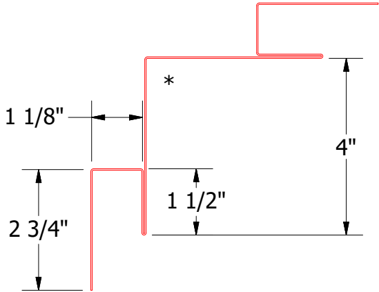
VSA601-Inside Corner Post
