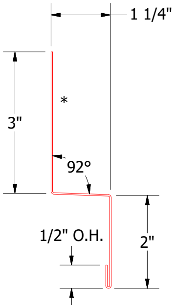
VSA550-Head Trim
