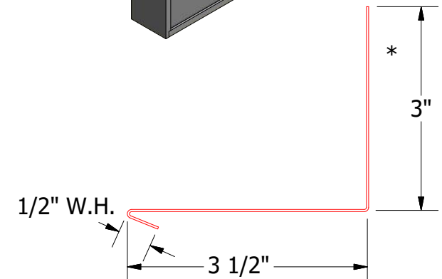
VSA683-Angle Trim with Return
