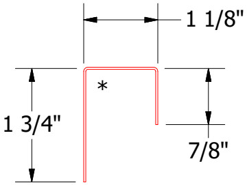
VSA270-J Closure
