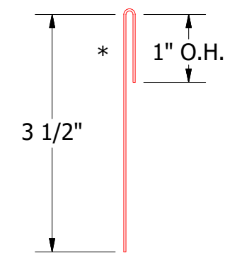
VSA962 - Utility Cleat without Return
