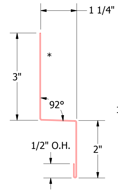
VSA550 - Head Trim
