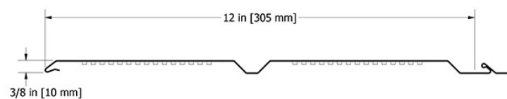
Wind-Lok Soffit Vented Panel (MPV120)
