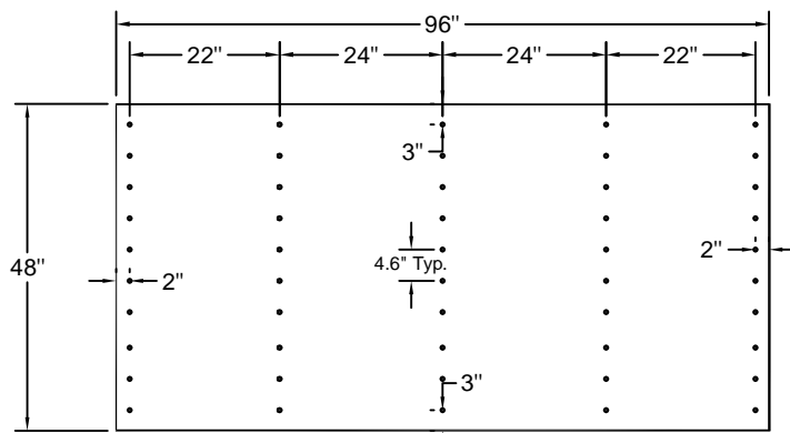
50 Fasteners per Board (4'x8')
