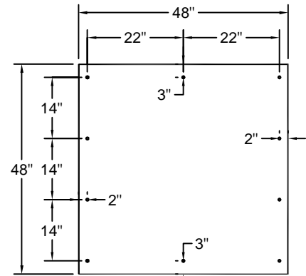
10 Fasteners per Board (4'x4')
