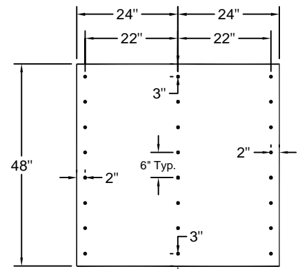
23 Fasteners per Board (4'x4')
