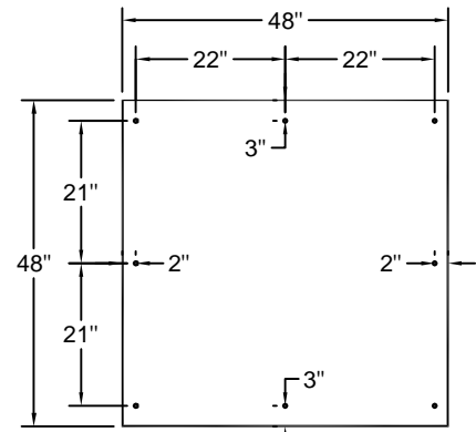
8 Fasteners per Board (4'x4')
