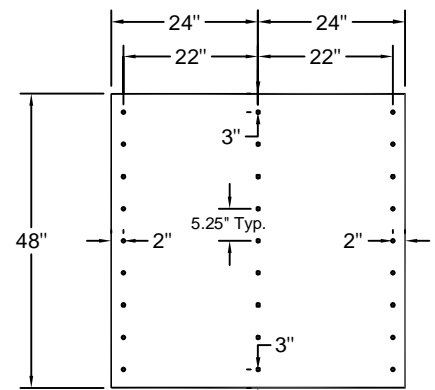
25 Fasteners per Board (4'x4')
