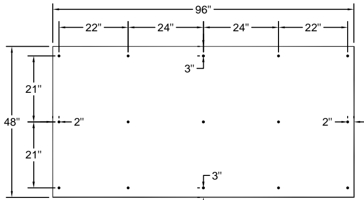
15 Fasteners per Board (4'x8')
