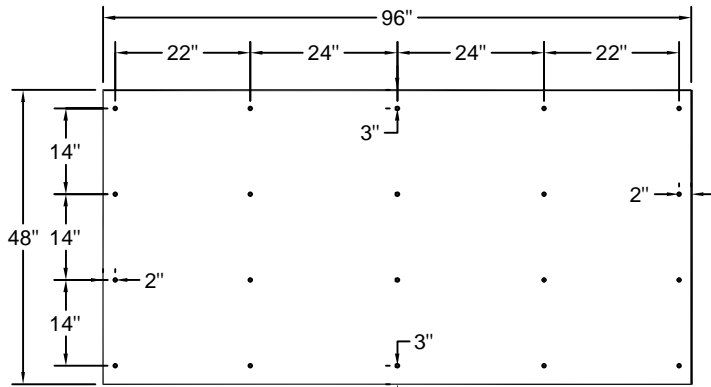
20 Fasteners per Board (4'x8')
