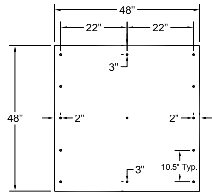
13 Fasteners per Board (4'x4')
