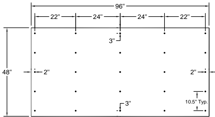
25 Fasteners per Board (4'x8')
