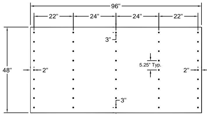
45 Fasteners per Board (4'x8')
