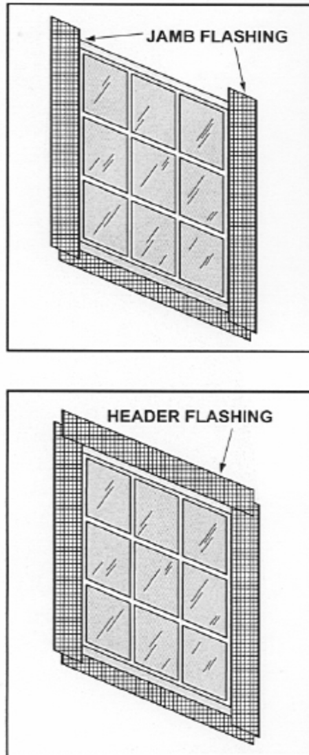
FIGURE 1—TYPICAL WINDOW FLASHING INSTALLATION
