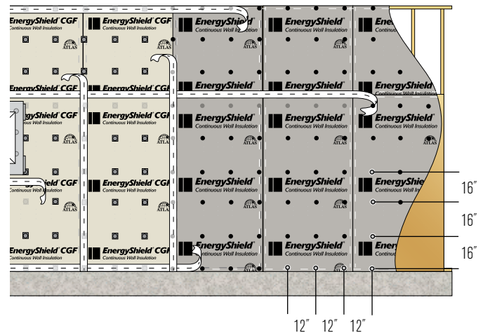
FIGURE B: FOAM BOARD AS CONTINUOUS INSULATION AND WRB OVER EXTERIOR WOOD SHEATHING FASTENED TO WOOD STUD FRAMING
