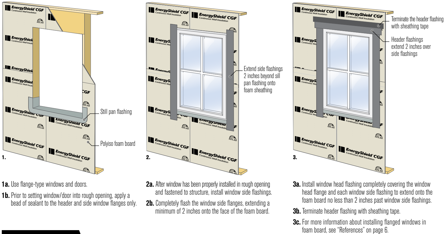
FIGURE C: FLANGED WINDOW INSTALLATION
