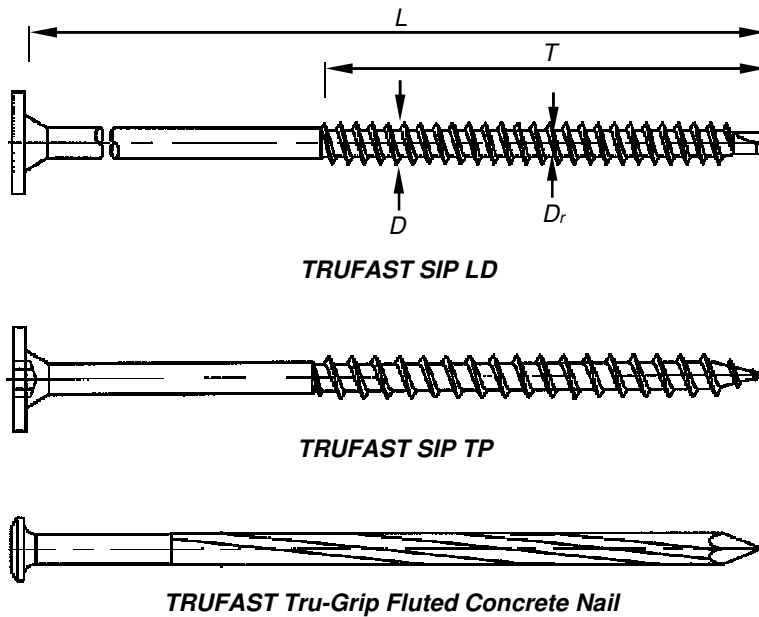
Figure 1: Fastener Geometry
