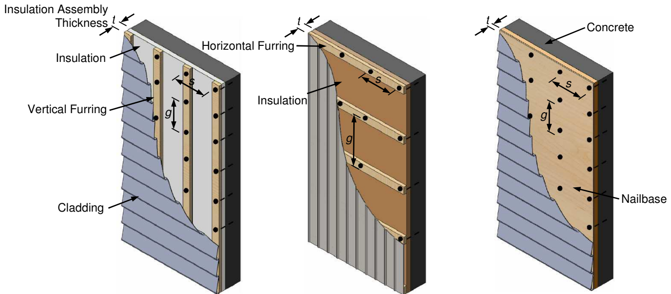
Figure 4: TRUFAST Tru-Grip into Concrete
