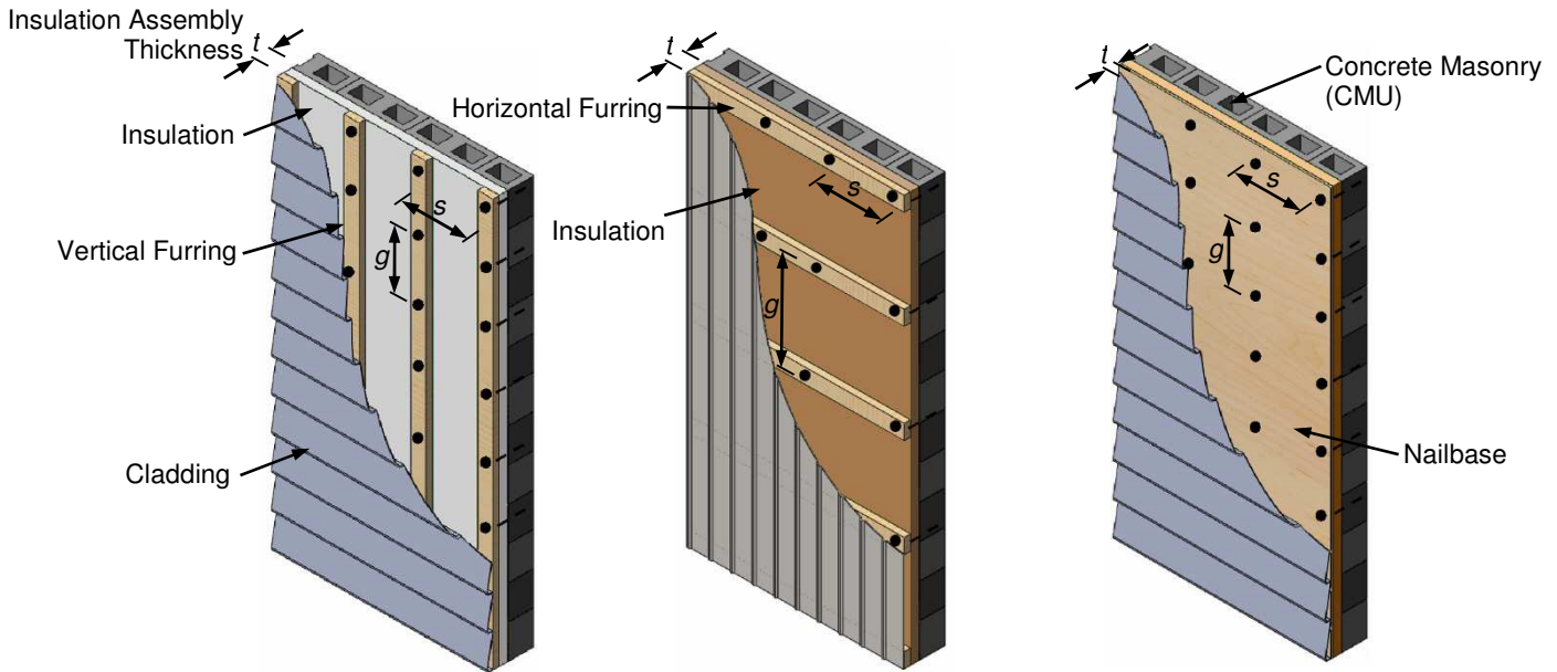
Figure 5: SIP LD into Concrete Masonry (CMU)
