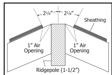
Ridgepole Diagram
