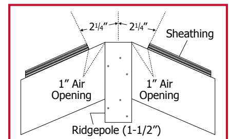
Ridgepole Diagram
