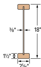
BCI® 60 Joists
