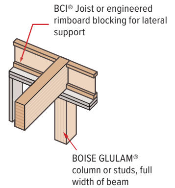
G03 Beam to Wall with Lateral Support
