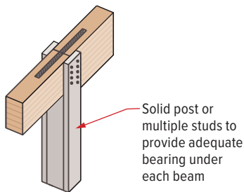
G08 Beam Depth Change at Intermediate Support
