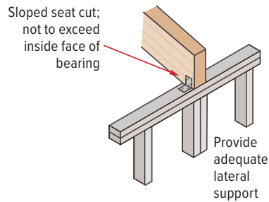
G09 Slope Seat Cut
