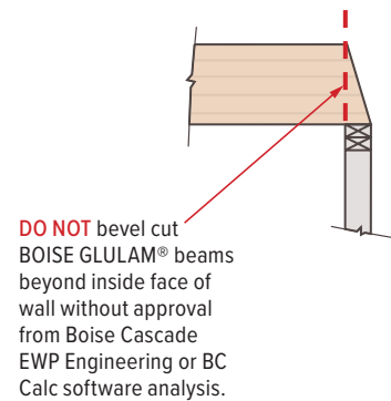
G10 Bevel Cut
