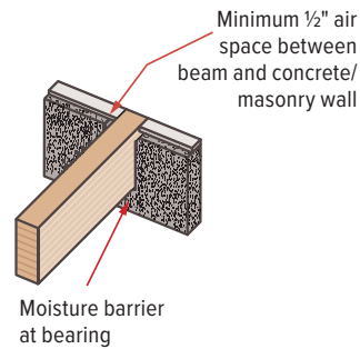
G06 Beam To Concrete/Masonry Walls
