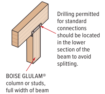
G07 Beam to Column Connection
