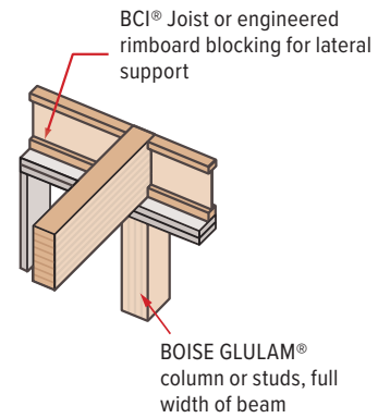
G03 Beam to Wall with Lateral Support
