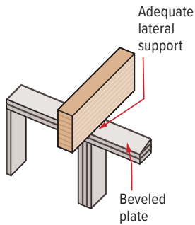
G04 End Wall Bevel Plate
