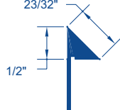
3/4" Chamfer Former w/Leg CL -750
