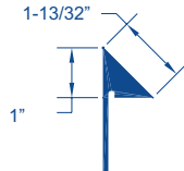
1-1/2" Chamfer Former w/Leg CL -1500
