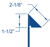
2" Chamfer Former w/Leg CL -2000
