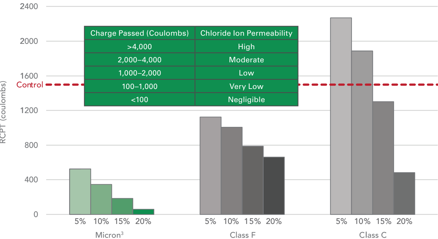
Figure 9: Rapid Chloride Permeability, 90 Days
