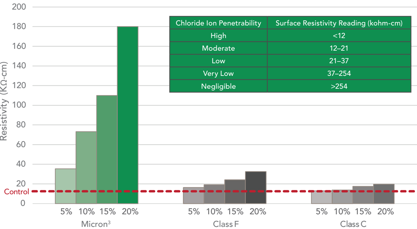
Figure 5: Concrete Resistivity, 90 Days
