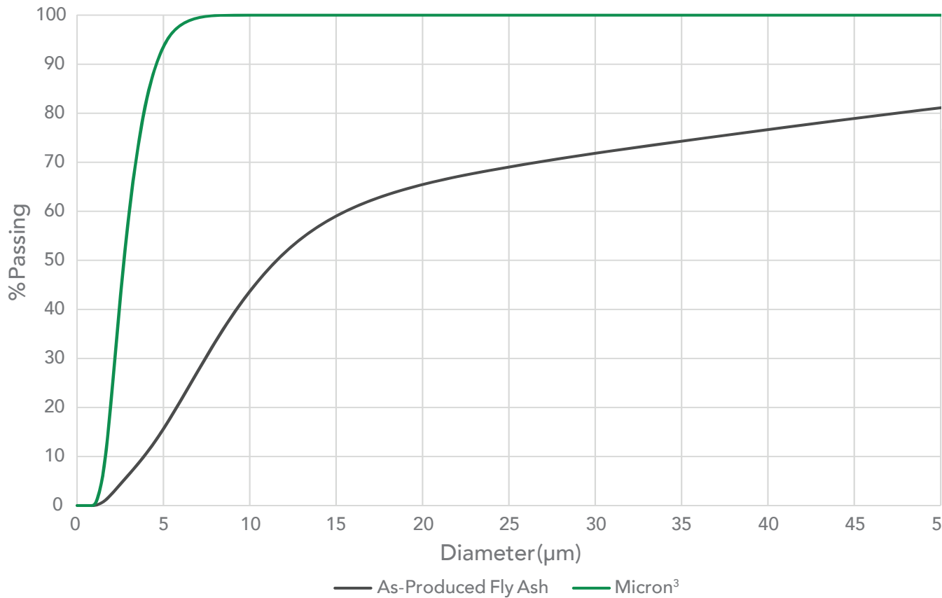
Figure 1: Particle Size Distribution of Micron3 Compared to As-Produced Fly Ash
