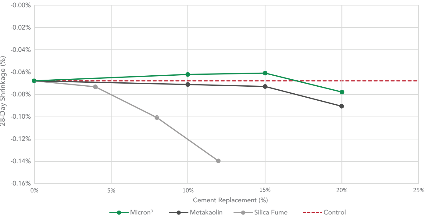
Figure 6: 28-Day Shrinkage of C157 Mortar Bars
