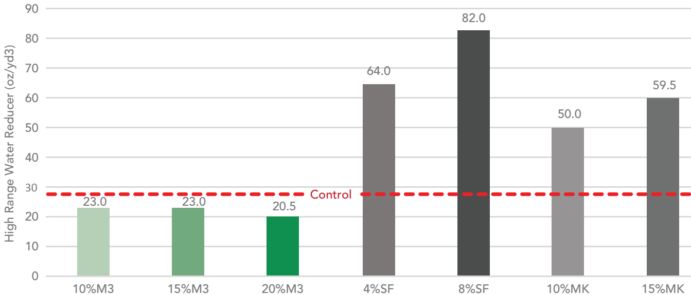
Figure 8: High Range Water Reducer Dosage
