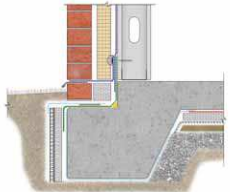
Below Grade to Wall Tie-In
