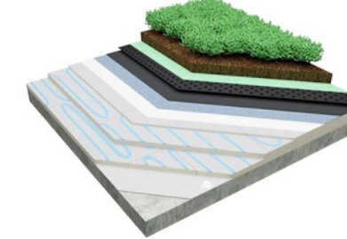
Traditional Roof Garden With FleeceBACK® KEE HP Membrane
