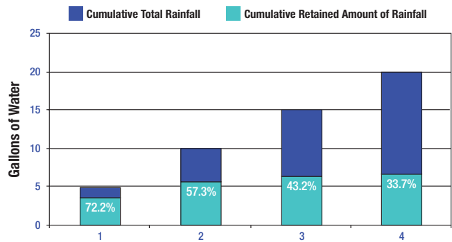
Cumulative Water Retention in a Four-Inch GreenGrid Unit During a Simulated Two-Hour Rain Storm
