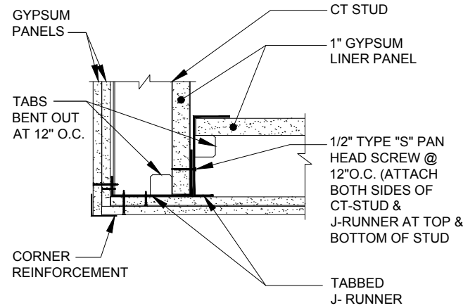
9 INSIDE CORNER
