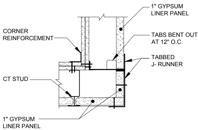
10 INSIDE CORNER
