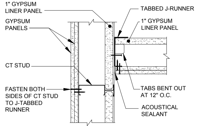
11 WALL JUNCTION
