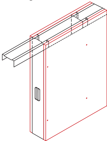
Non-Composite | Fully Braced Gypsum Board Full Height Both Sides
