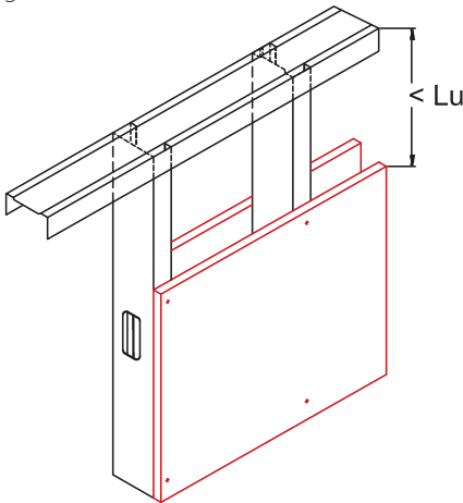
Non-Composite | Fully Braced Unbraced Length is Less Than L_u
