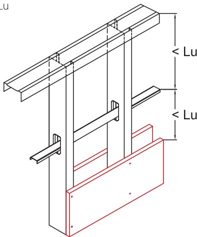
Non-Composite | Fully Braced Bracing Spacing Above Gypsum is Less Than L_u
