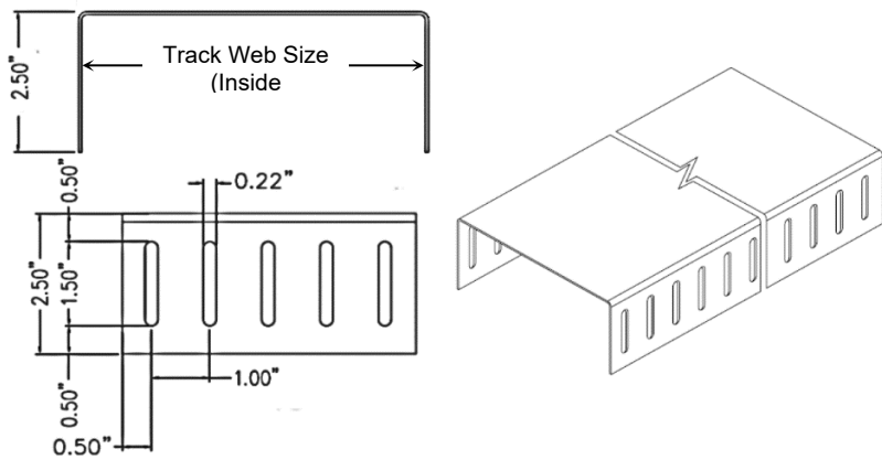
TRACK (Slotted Flange) xxxCST250 or xxxSLT250
