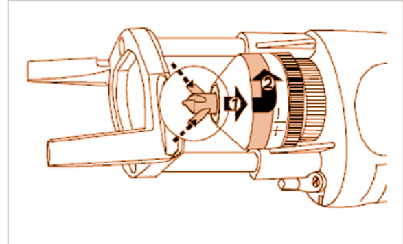
Figure 13.4: Retracting the forming pins
