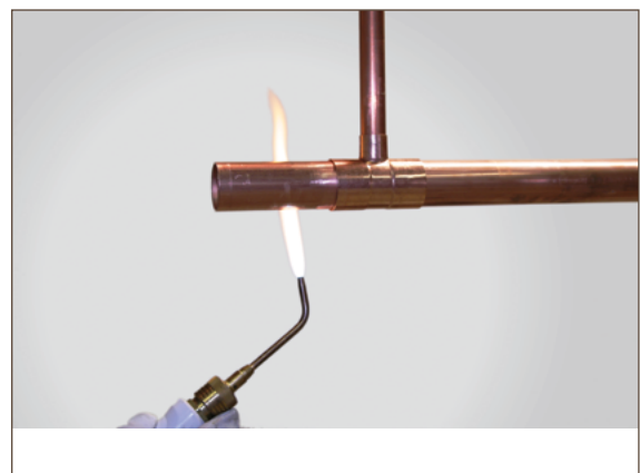
Figure 7.13. Preheating Tube
