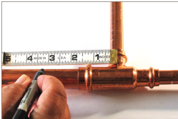
Figure 11.5. Measuring
