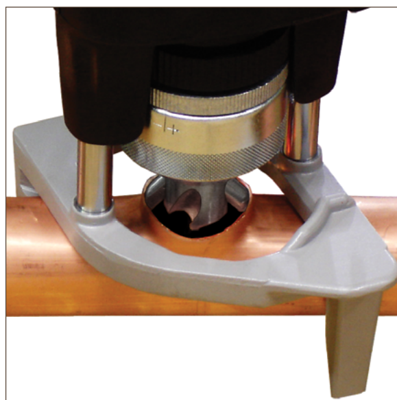
Figure 13.7. Forming the outlet
