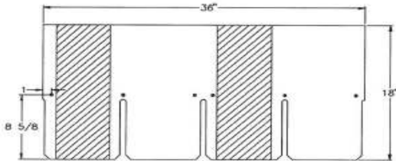
Detail B Overall Dimensions and Nailing Pattern
