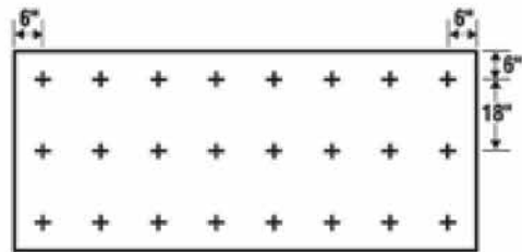
24 Fasteners/Board
