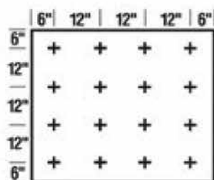
16 Fasteners/Board
