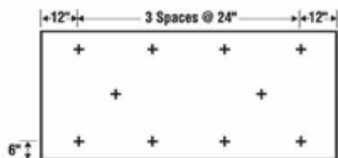
10 Fasteners/Board
