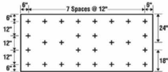
28 Fasteners/Board
