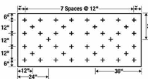
42 Fasteners/Board
