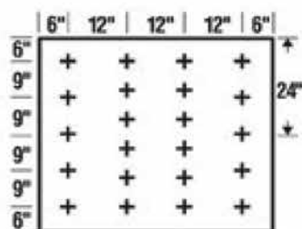
22 Fasteners/Board
