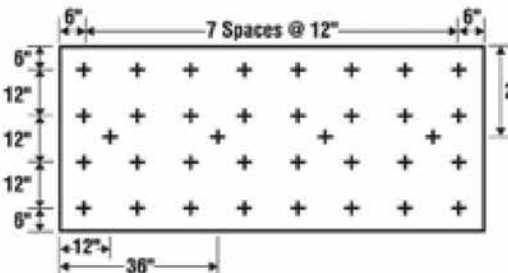
36 Fasteners/Board
