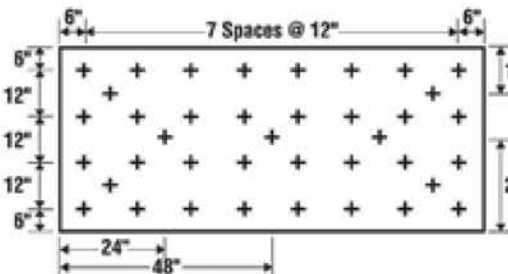
39 Fasteners/Board
