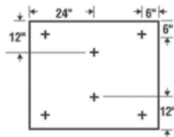
6 Fasteners/Board
