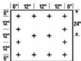
14 Fasteners/Board
