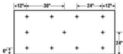
11 Fasteners/Board
