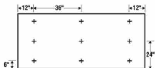
9 Fasteners/Board
