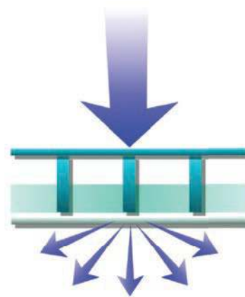
Figure 14: Floor/ceiling assembly with carpet and pad, particle board underlayment, plywood subfloor, resilient channels and gypsum board ceiling, with fiberglass insulation in joist cavities. STC = 53; IIC = 73.
