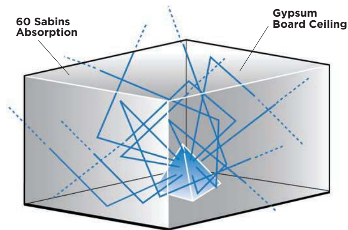
Figure 17: Room attenuation with gypsum board ceiling = 60 sabins at 250 Hz.
