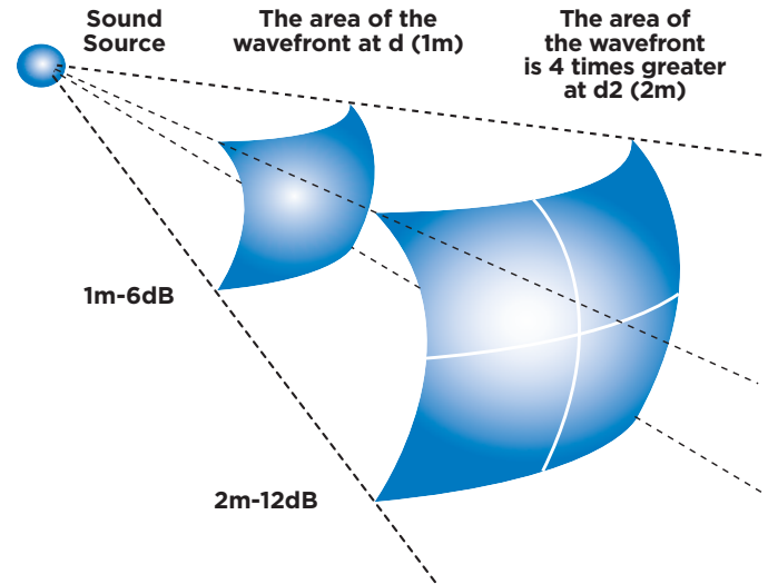
Figure 8: Direct sound energy decreases with the square of the distance from the source
