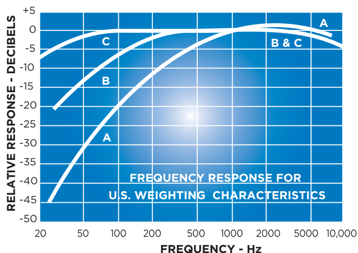
Figure 7: A, B, and C frequency weighting curves
