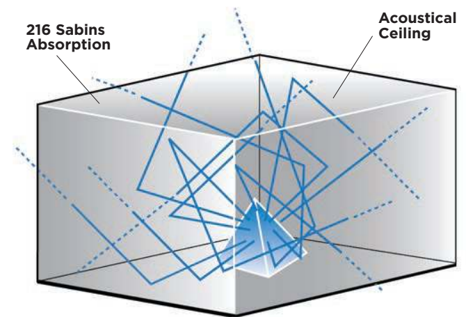
Figure 18: Acoustical ceiling adds 156 sabins, reduces noise level 5.5 dB.
