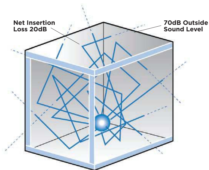
Figure 16: Noise enclosure without interior sound absorption. Exterior sound level is 70 dB.
