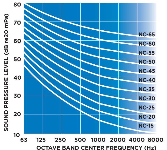
Figure 9: Noise criteria curves for octave band center frequencies from 63 Hz to 8000 Hz.
