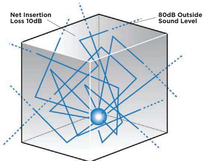
Figure 15: Noise enclosure without interior sound absorption. Exterior sound level is 80 dB.
