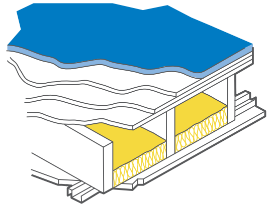
Figure 14: Floor/ceiling assembly with carpet and pad, particle board underlayment, plywood subfloor, resilient channels and gypsum board ceiling, with fiberglass insulation in joist cavities. STC = 53; IIC = 73.
