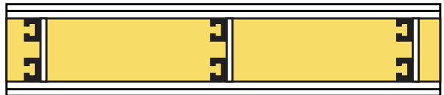
Rating: 1 hour non-bearing (U436) Chase wall: Double layer 5/8" CertainTeed Type X 1-5/8" steel studs on 24" centers CertainTeed fiberglass insulation to fill cavity
