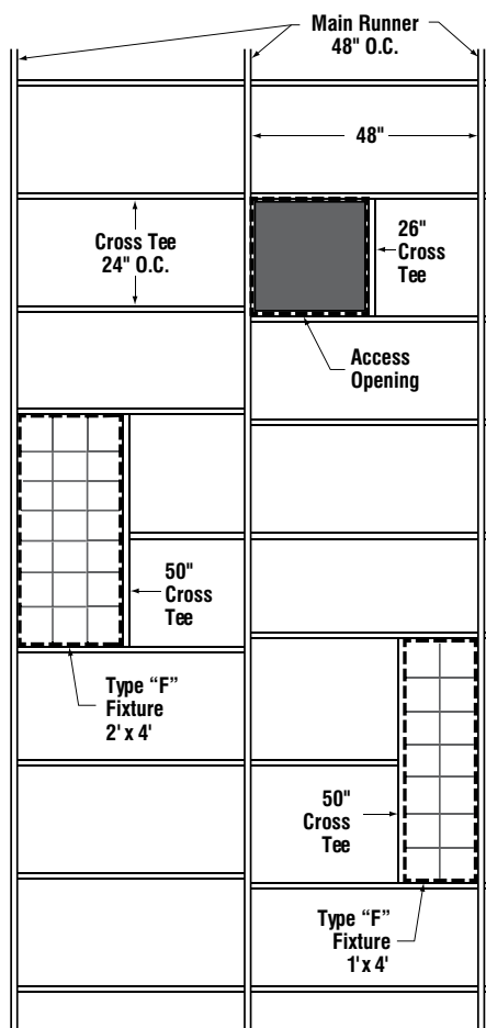
Grid for 48" Type F Fixture
