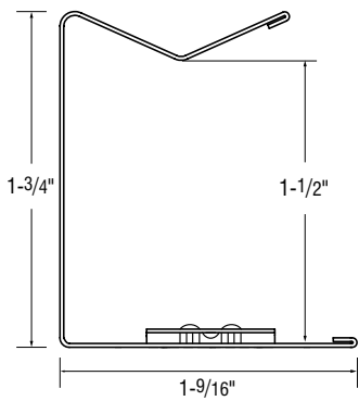
Spacing (side view)
