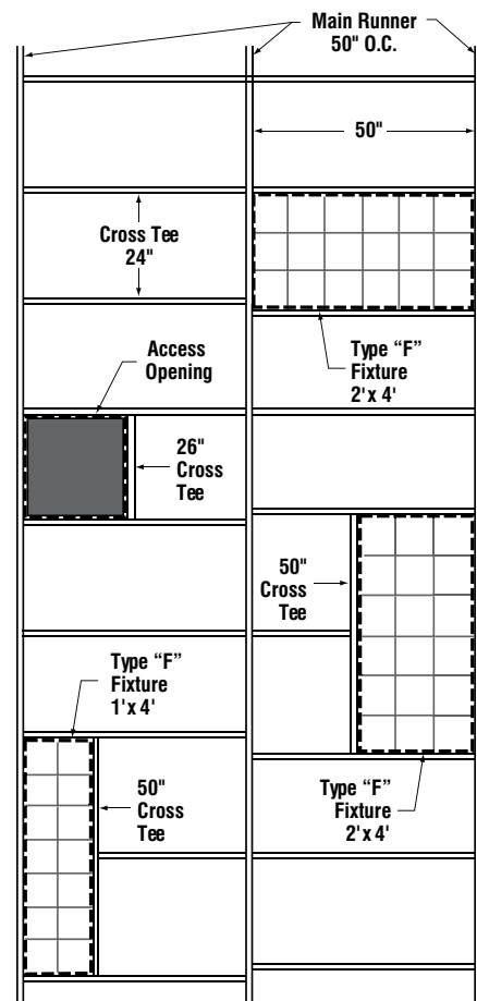
Grid for 50" Type F Fixture
