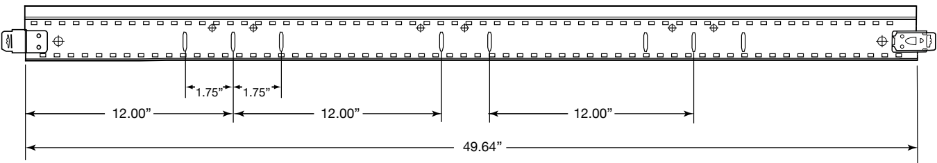
50" Cross Tee DWS4.16-30-20
