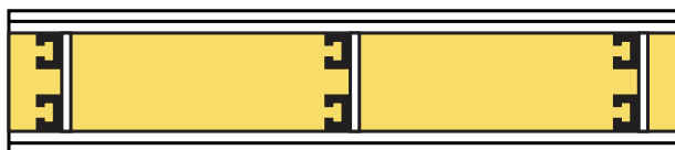
Rating: 1 hour non-bearing (U436) Chase wall: Double layer 5/8" CertainTeed Type X 1-5/8" steel studs on 24" centers CertainTeed fiberglass insulation to fill cavity
